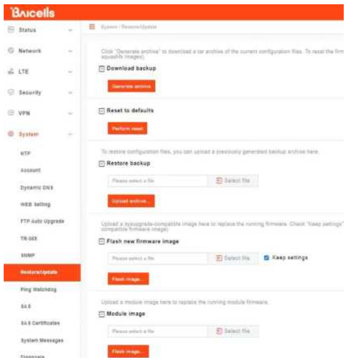
Figure 3-50 Restore/Update
