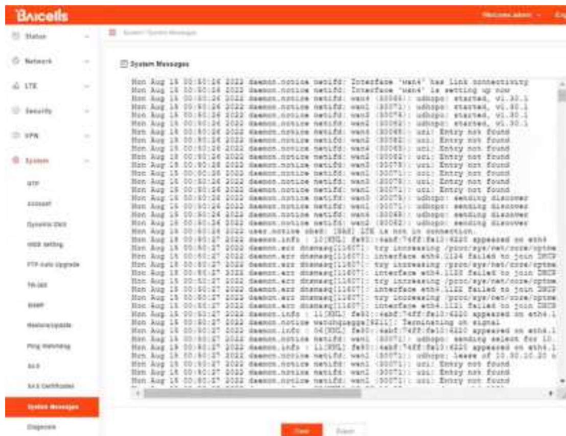
Figure 3-58 System Messages
