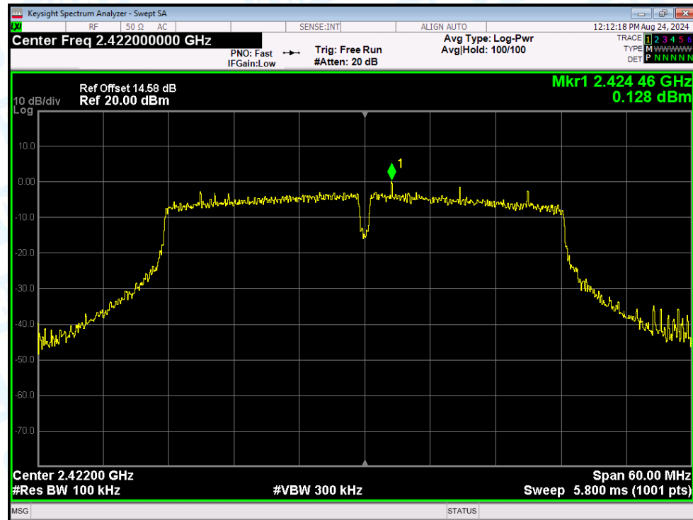
Band Edge NVNT ax(VHT40) 2422MHz Ant3 Emission
