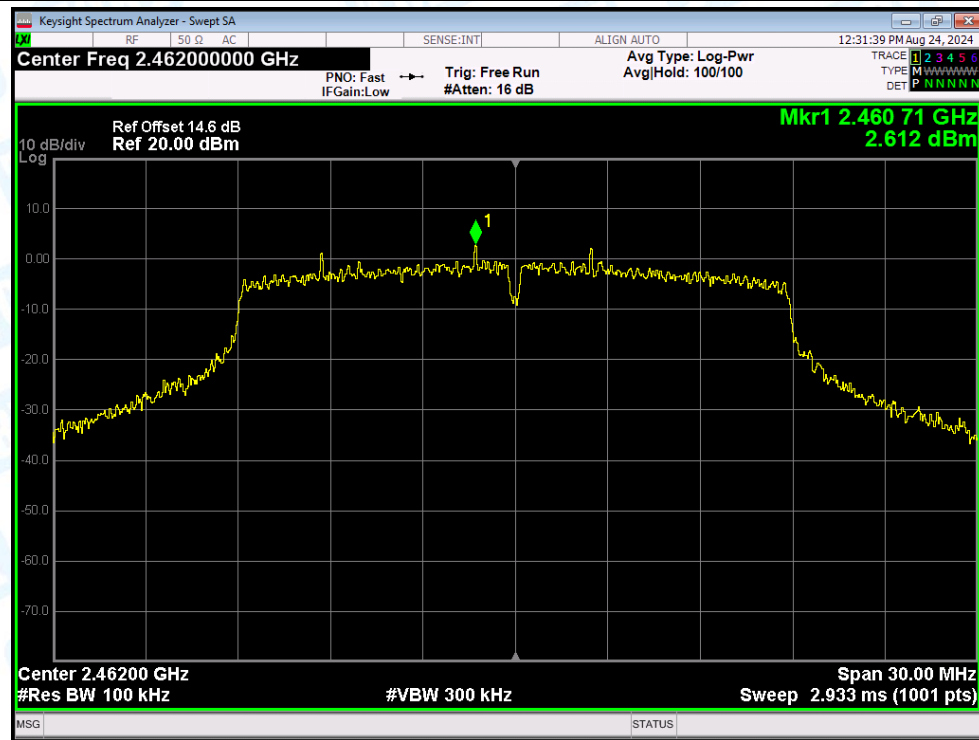
Tx. Spurious NVNT n(HT20) 2462MHz Ant3 Emission
