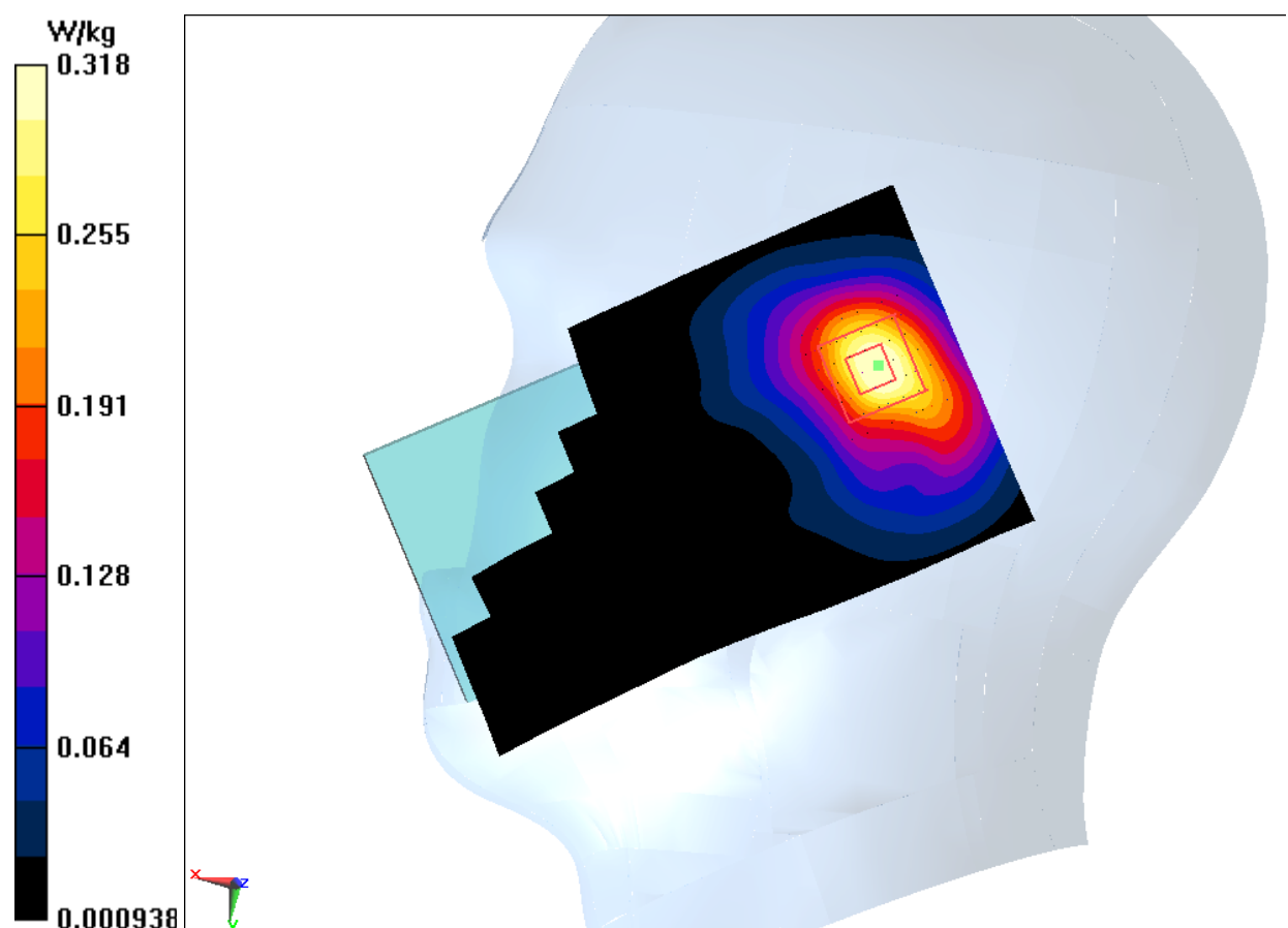
Fig.15 2450 MHz
