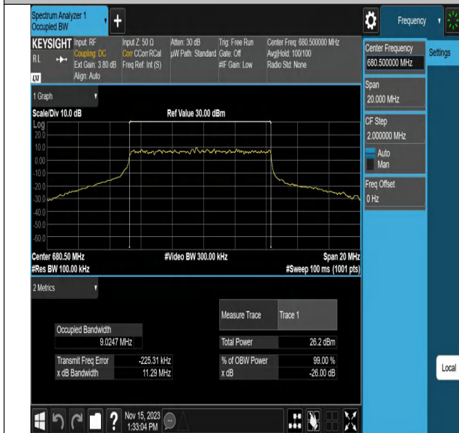
NTNV_N71_PC3_15_10_M_TID3_Ant1#1
