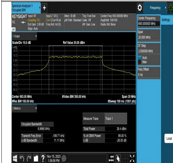
NTNV_N71_PC3_15_10_H_TID3_Ant1#1
