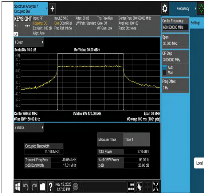
NTNV_N71_PC3_15_15_M_TID5_Ant1#1
