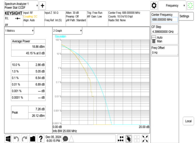
Band71_20MHz_256QAM_RB100_0_CH133372
