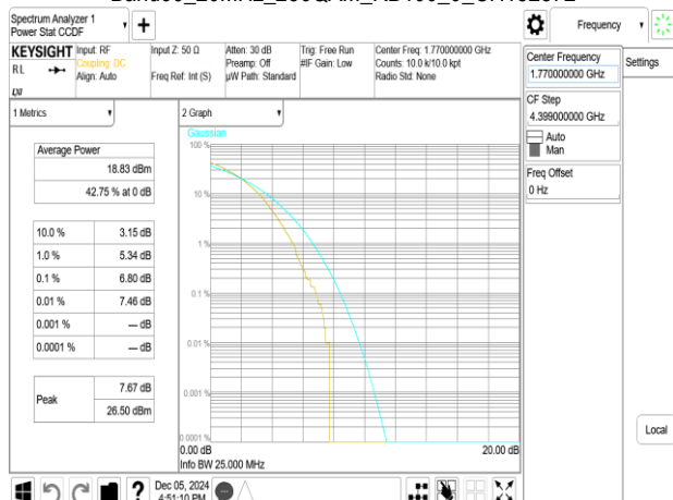
Band66_20MHz_256QAM_RB100_0_CH132572
