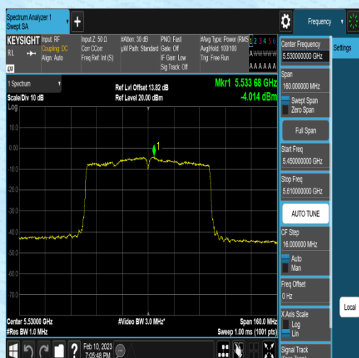
11AC80MIMO-Ant1-5530--5.07-1.06-0.00-0.00
