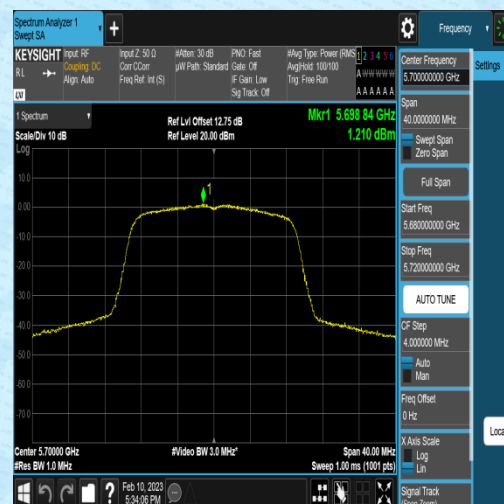
11AC20MIMO-Ant2-5700-0.96-0.25-0.00-0.00
