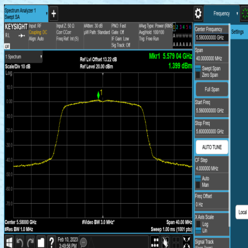
11N20MIMO-Ant1-5580-1.27-0.13-0.00-0.00
