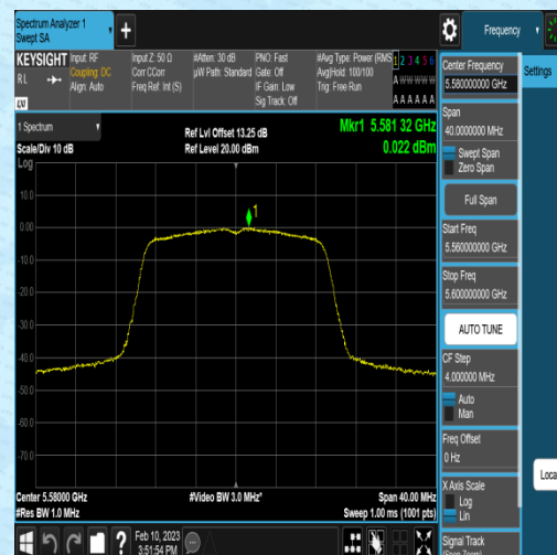
11N20MIMO-Ant2-5580--0.14-0.16-0.00-0.00
