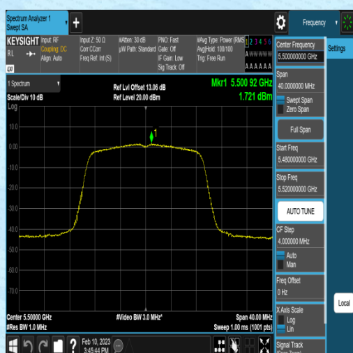
11N20MIMO-Ant1-5500-1.56-0.16-0.00-0.00
