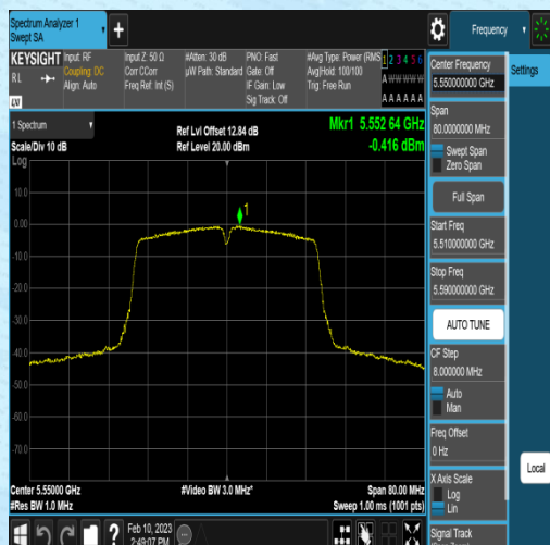
11AC40SISO-Ant2-5550--0.68-0.26-0.00-0.00
