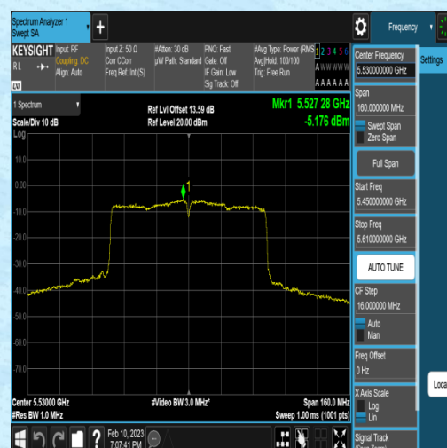
11AC80MIMO-Ant2-5530--6.01-0.83-0.00-0.00
