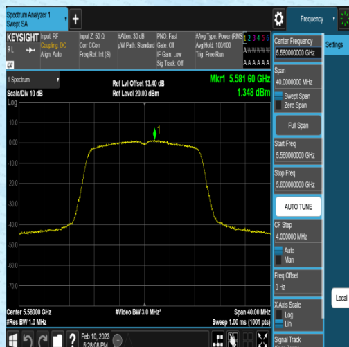
11AC20MIMO-Ant1-5580-1.04-0.31-0.00-0.00
