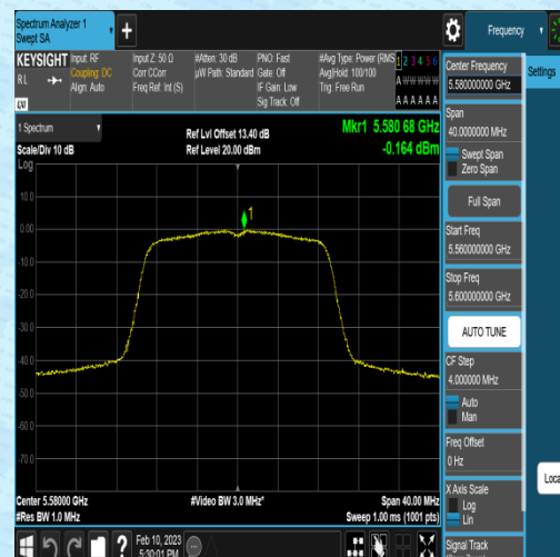
11AC20MIMO-Ant2-5580--0.47-0.31-0.00-0.00
