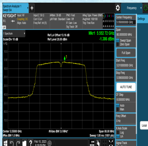
11AC40MIMO-Ant1-5550--1.97-0.58-0.00-0.00
