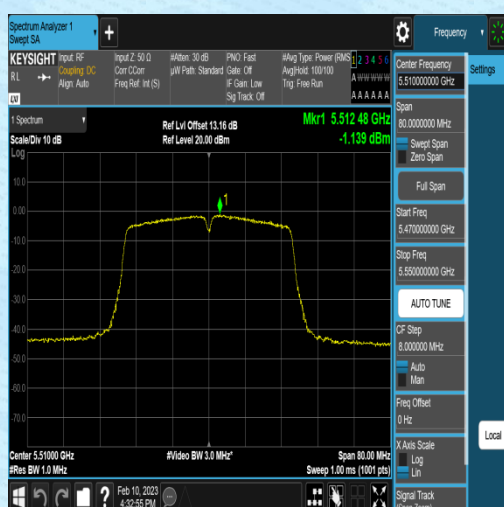
11N40MIMO-Ant1-5510--1.40-0.26-0.00-0.00
