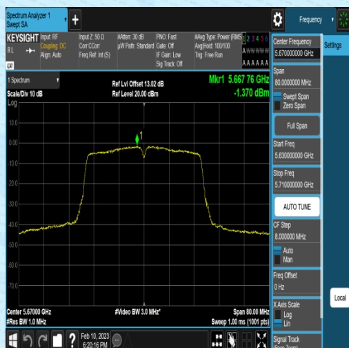
11AC40MIMO-Ant1-5670--1.84-0.47-0.00-0.00
