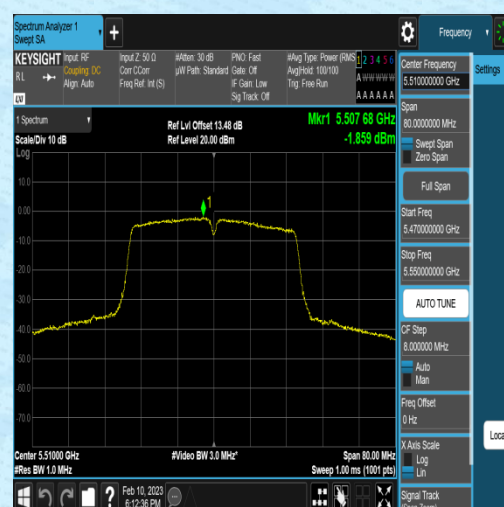
11AC40MIMO-Ant2-5510--2.44-0.58-0.00-0.00
