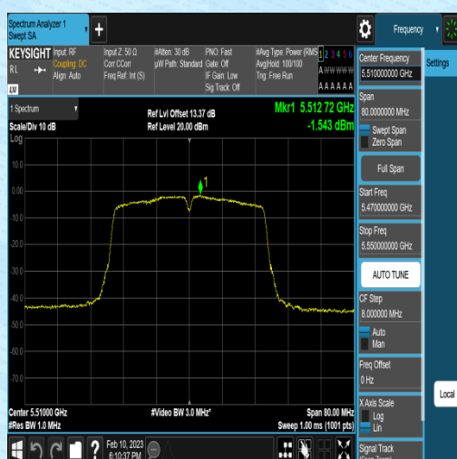
11AC40MIMO-Ant1-5510--2.01-0.47-0.00-0.00
