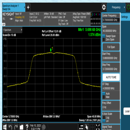
11AC20MIMO-Ant1-5700-1.26-0.31-0.00-0.00
