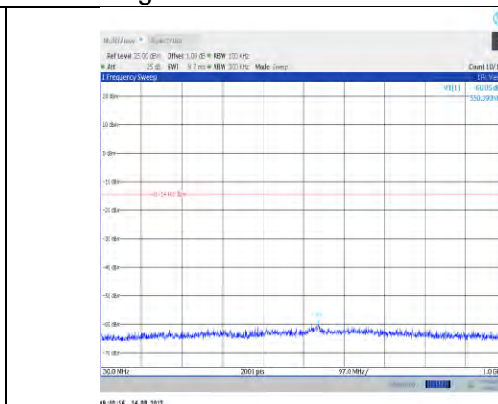
11g-CDD-Ant10-2462-30~1000
