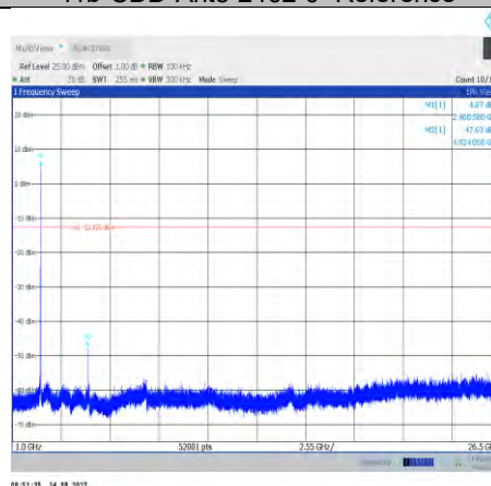
11b-CDD-Ant8-2462-1000~26500
