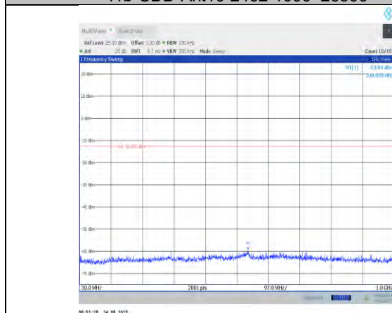
11b-CDD-Ant8-2462-30~1000
