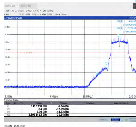
11g-CDD-Ant8-2412
