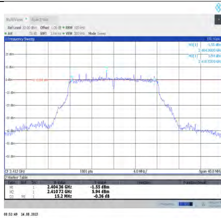
11g-CDD-Ant10-2412
