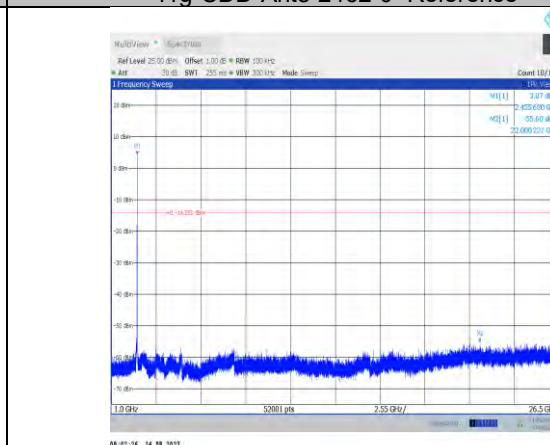
11g-CDD-Ant8-2462-1000~26500
