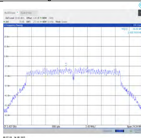
11g-CDD-Ant8-2437
