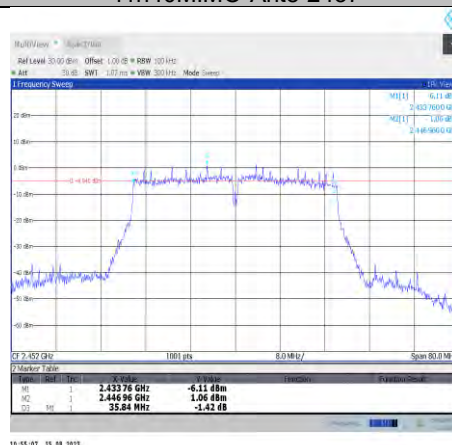
11n40MIMO-Ant8-2452
