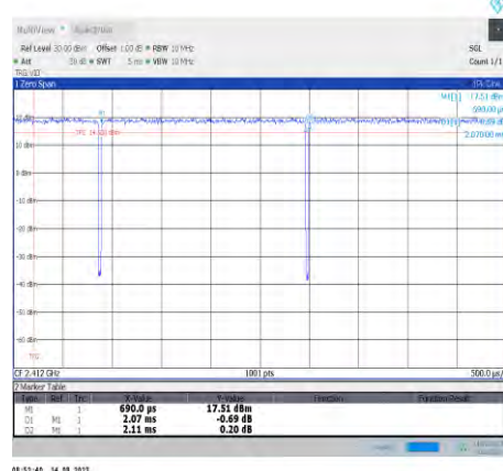
NTNV-11q-CDD-Ant10-2412
