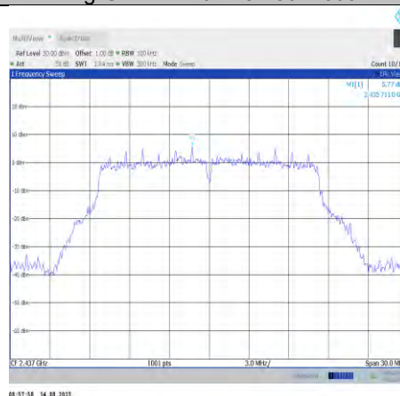
11g-CDD-Ant8-2437-0~Reference
