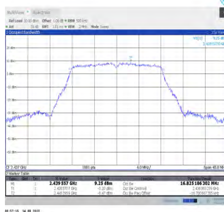
11g-CDD-Ant8-2437
