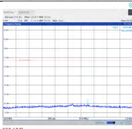
11b-CDD-Ant8-2437-30~1000
