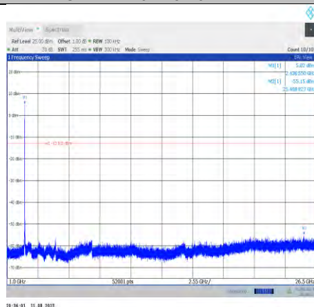
11b-CDD-Ant10-2437-1000~26500
