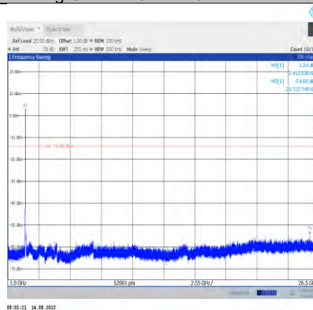
11g-CDD-Ant8-2412-1000~26500
