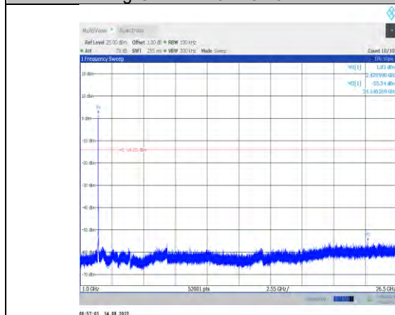
11g-CDD-Ant10-2437-1000~26500
