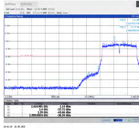
11n40MIMO-Ant8-2422
