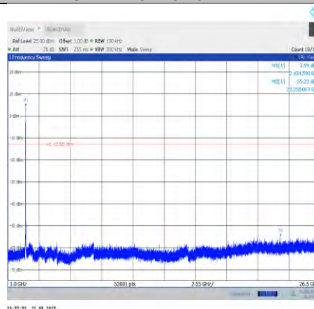
11b-CDD-Ant8-2437-1000~26500
