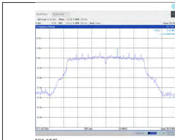
11g-CDD-Ant10-2412-0~Reference
