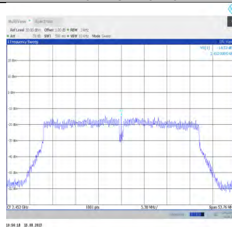
11n40MIMO-Ant8-2452
