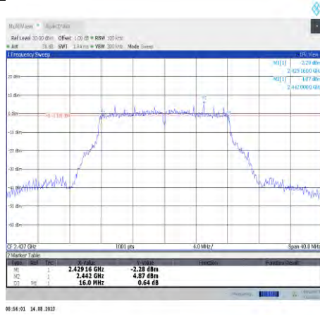
11g-CDD-Ant10-2437
