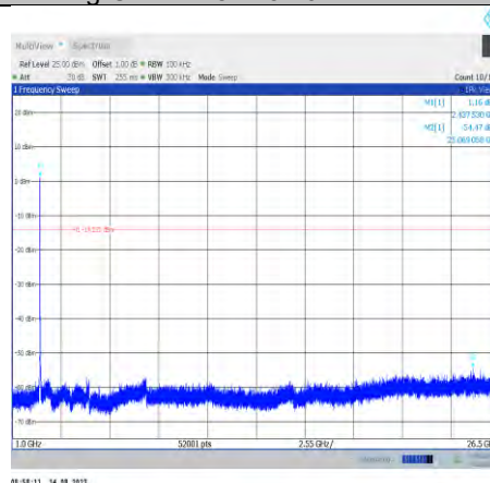
11g-CDD-Ant8-2437-1000~26500
