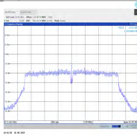
11n40MIMO-Ant8-2422
