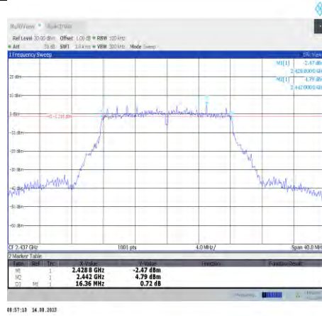
11g-CDD-Ant8-2437
