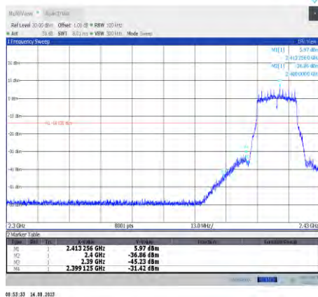
11g-CDD-Ant10-2412
