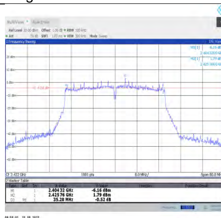
11n40MIMO-Ant8-2422
