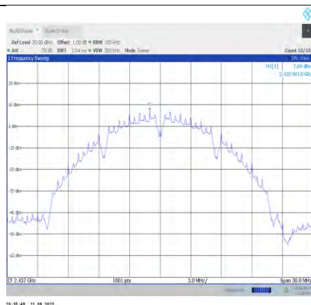
11b-CDD-Ant10-2437-0~Reference
