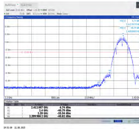
11b-CDD-Ant8-2412
