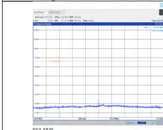
11g-CDD-Ant8-2412-30~1000
