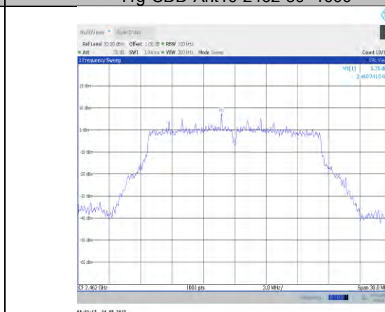
11g-CDD-Ant8-2462-0~Reference
