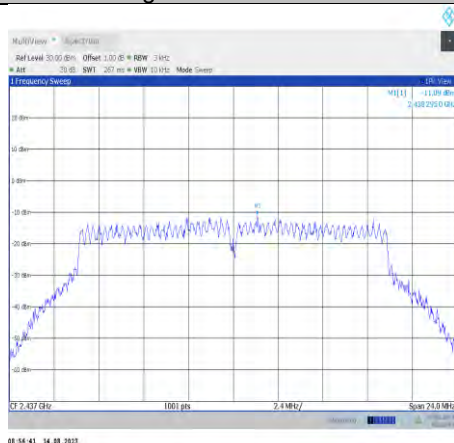
11g-CDD-Ant10-2437
