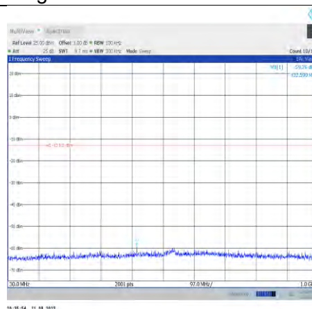
11b-CDD-Ant10-2437-30~1000
