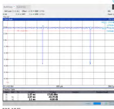
NTNV-11q-CDD-Ant8-2412
