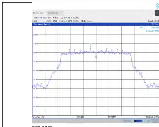
11g-CDD-Ant10-2437-0~Reference
