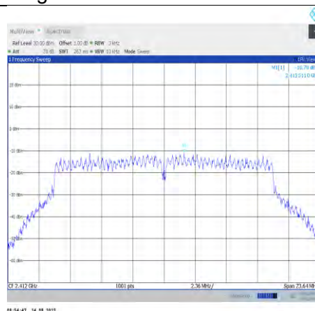
11g-CDD-Ant8-2412
