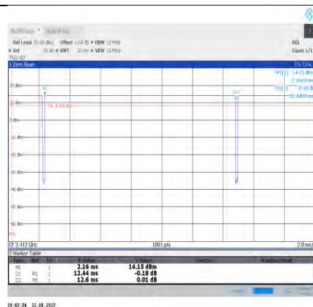
NTNV-11b-CDD-Ant10-2412
