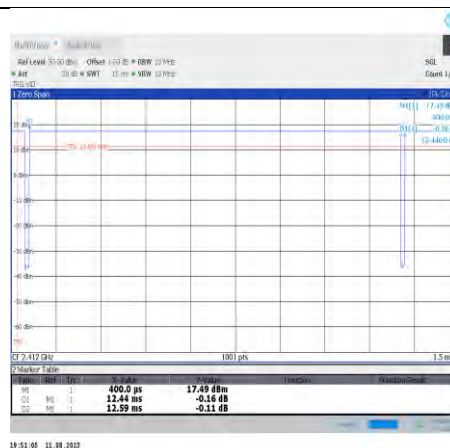
NTNV-11b-CDD-Ant8-2412
