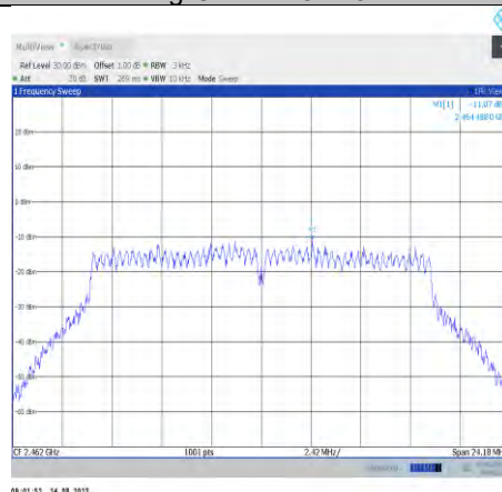
11g-CDD-Ant8-2462
