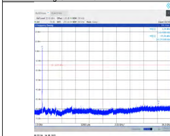
11g-CDD-Ant10-2412-1000~26500
