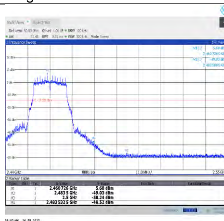
11g-CDD-Ant8-2462
