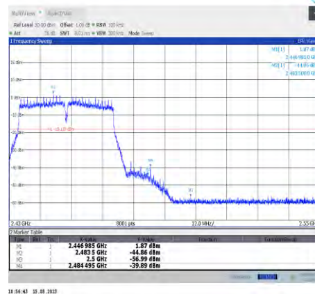
11n40MIMO-Ant8-2452
