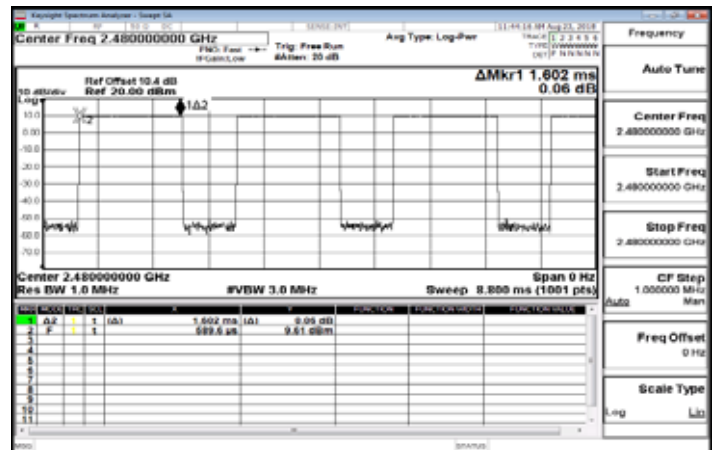
Dwell Time_GFSK_1M_DH3_2480MHz
