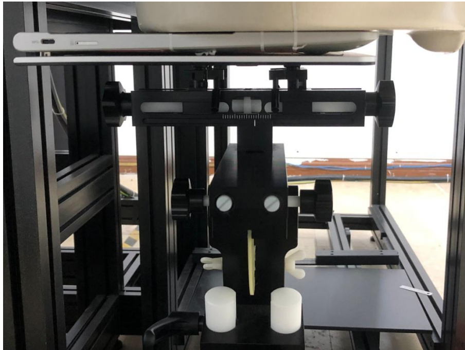
Front Surface of Keyboard (Test distance: 0mm)
