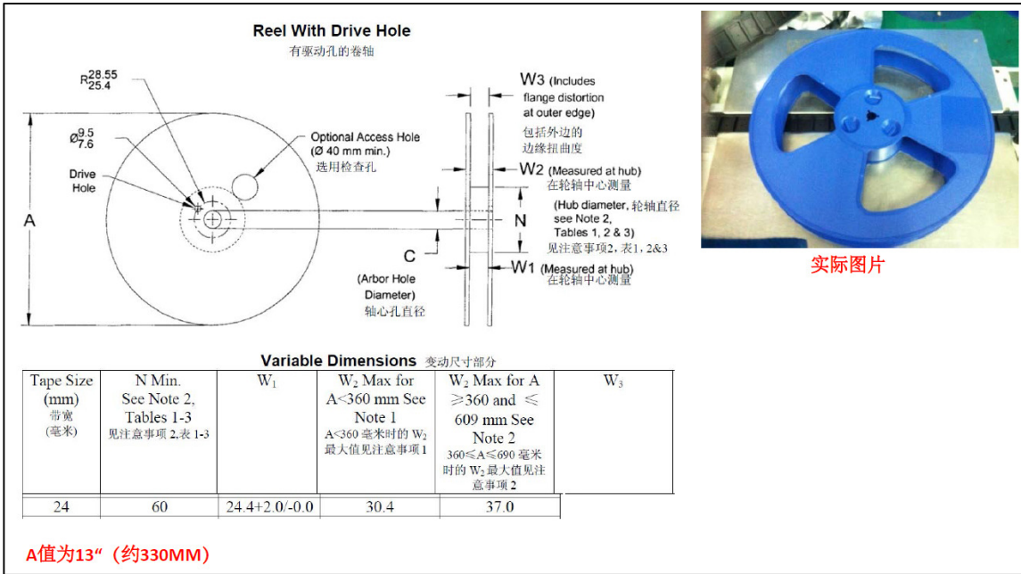
Figure 17: Reel specifications
