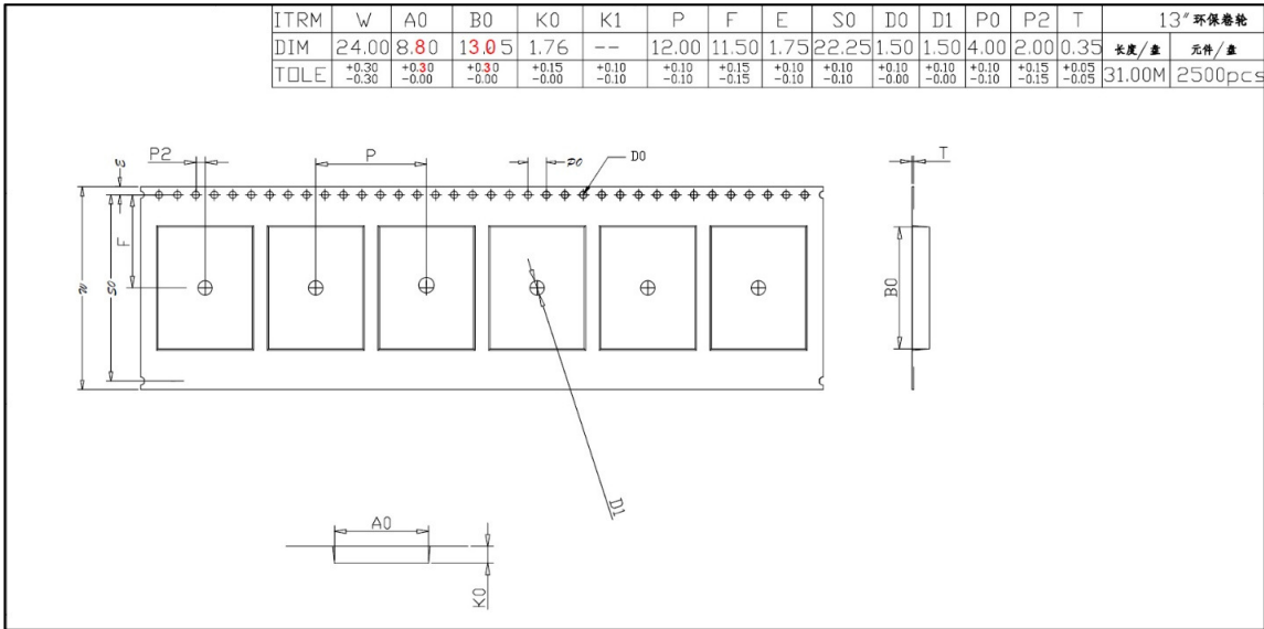
Figure 18: Tape specifications
