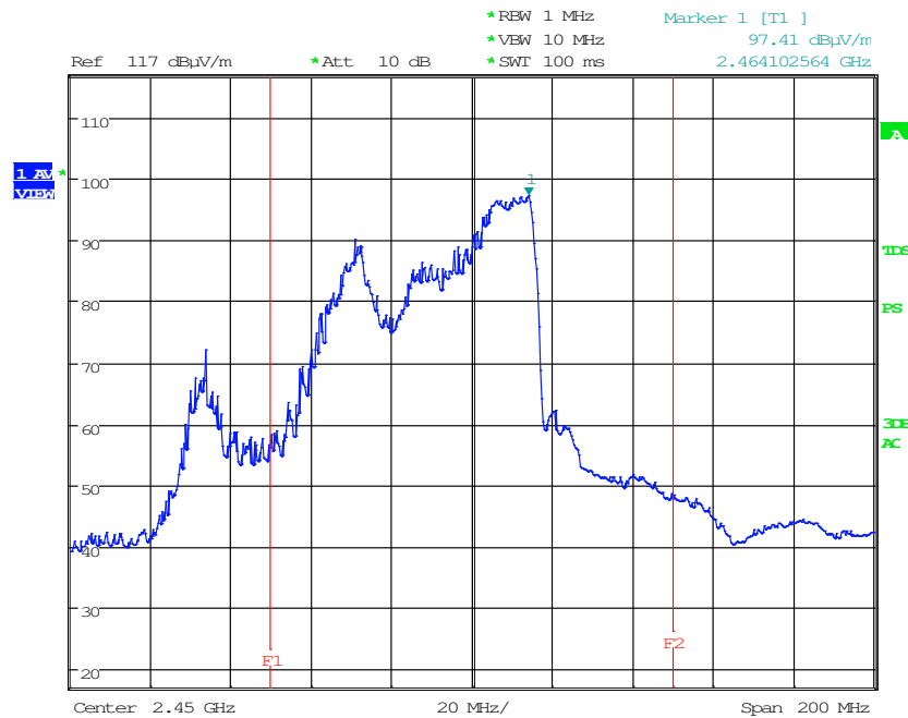
< Fig 7. Frequency Measurements (Maximum Frequency Observed: 2.464 GHz) >
