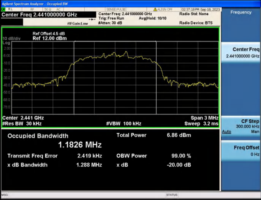
-20dB_Bandwidth_NVNT_ANT1_3-DH5_2441
