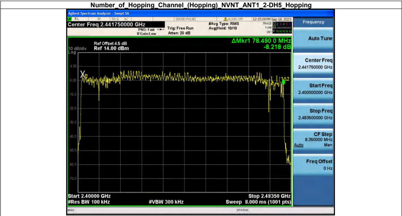
Number_of_Hopping_Channel_(Hopping)_NVNT_ANT1_2-DH5_Hopping
