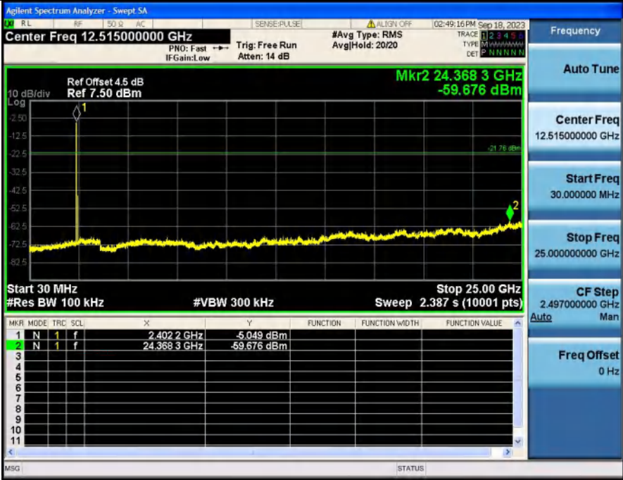
2_Spurious_Emissions_NVNT_ANT1_2-DH5_2402
