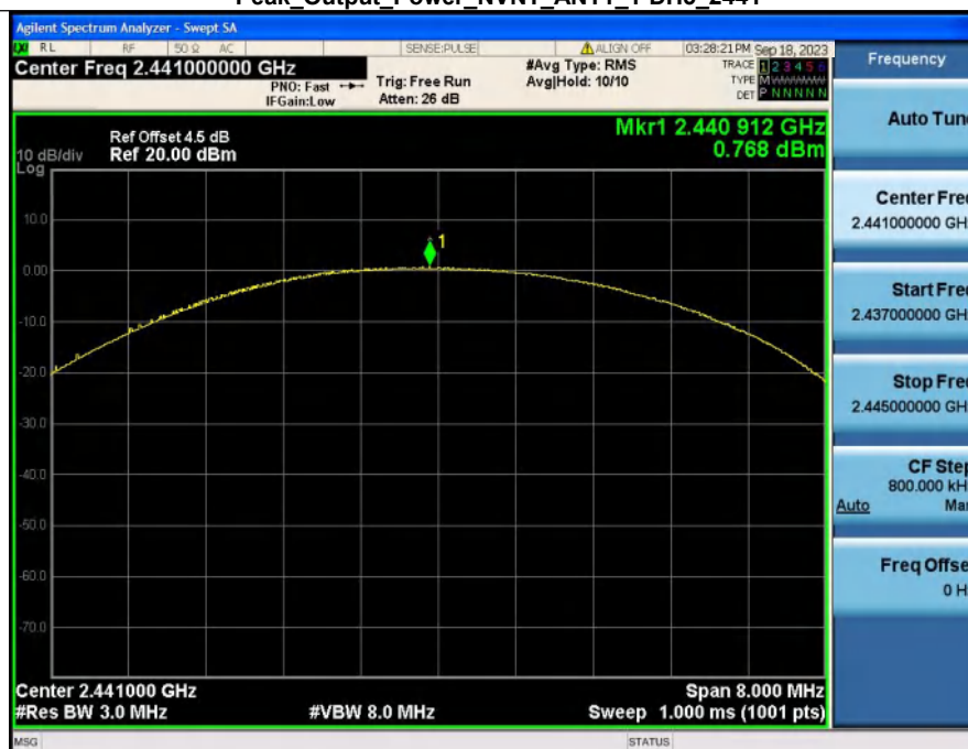
Peak_Output_Power_NVNT_ANT1_1-DH5_2441
