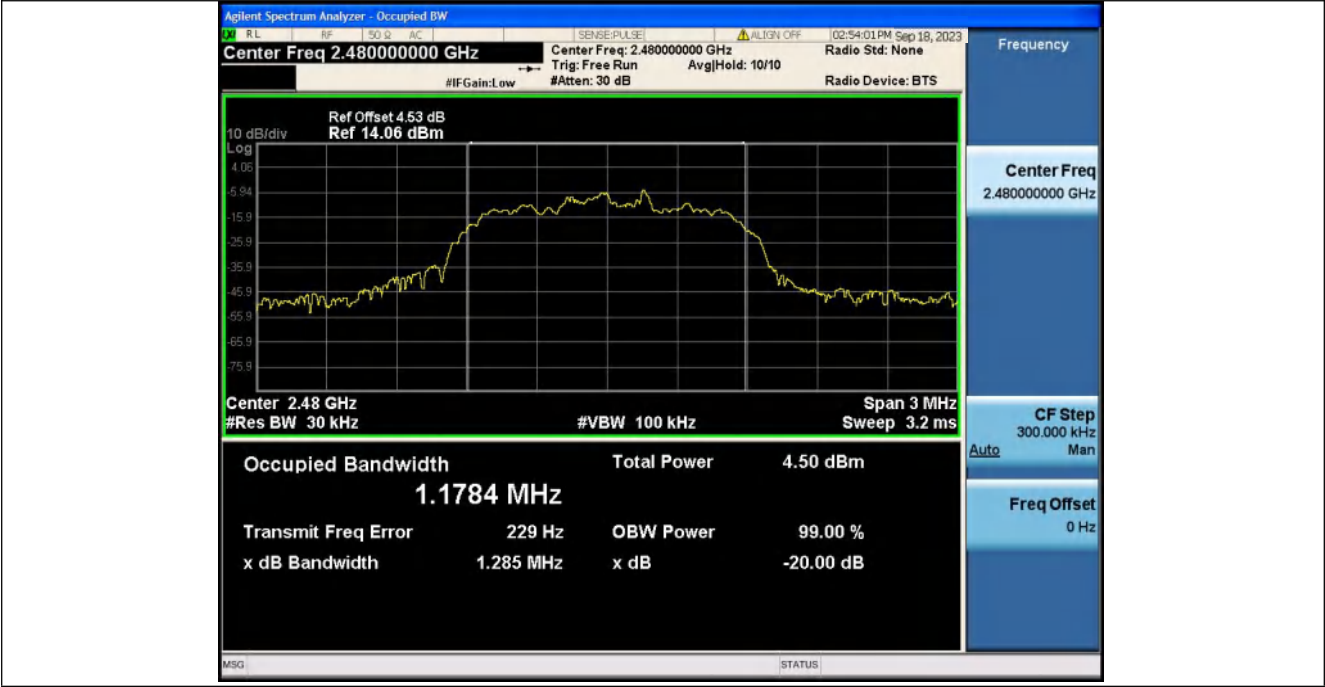
-20dB_Bandwidth_NVNT_ANT1_2-DH5_2480
