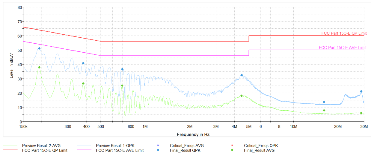
Plot 7-33. AC Line Conducted Plot with Bluetooth LE (N, 1Mbps – Ch.39, with AC/DC Adapter)
