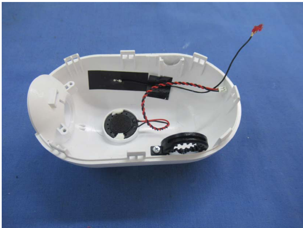
FPC Antenna
