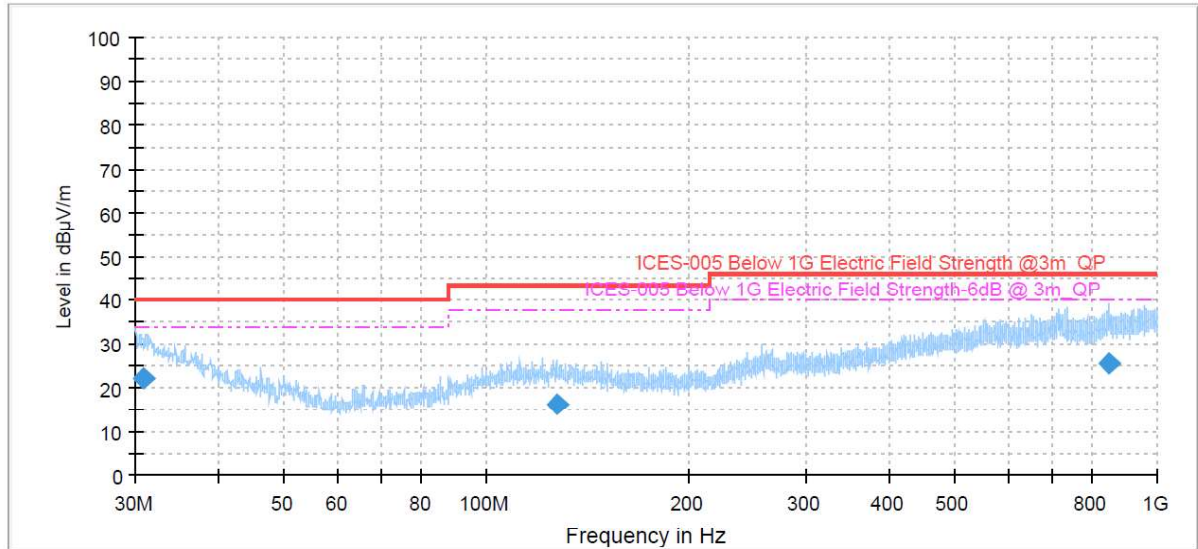
Figure 4: Spectral Diagrams, Radiated Emission, 30MHz-1000MHz, Vertical polarization
