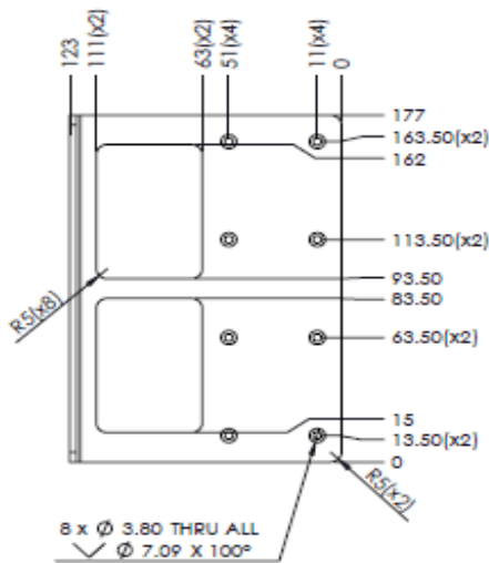
Figure 3-5. Top View of Brackets
