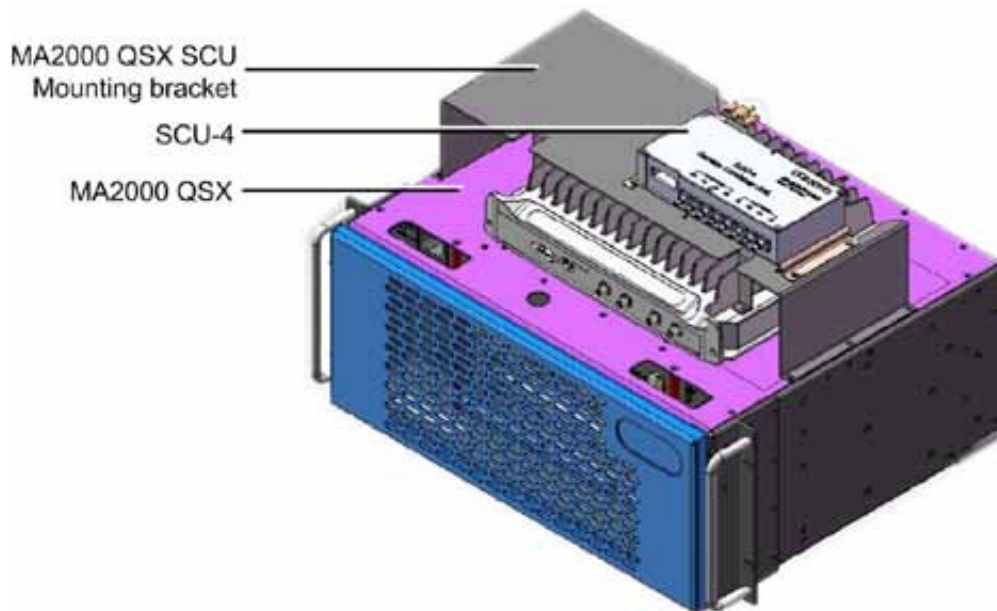
Figure 3-4. SCU-4 Mounted on QSX Unit
