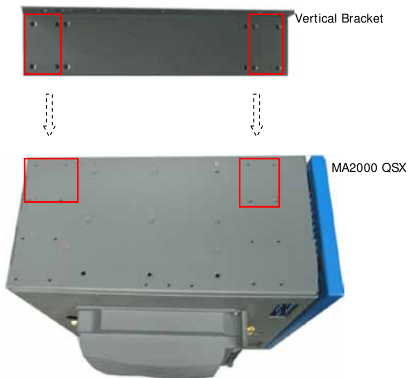
Figure 3-13. Location Assembly of Bracket on Enclosure
