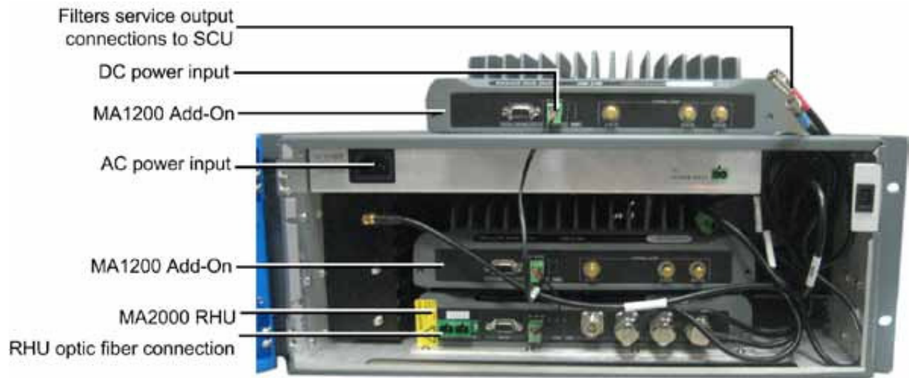
Figure 2-3. MA2000 QSX Open Cabinet View
