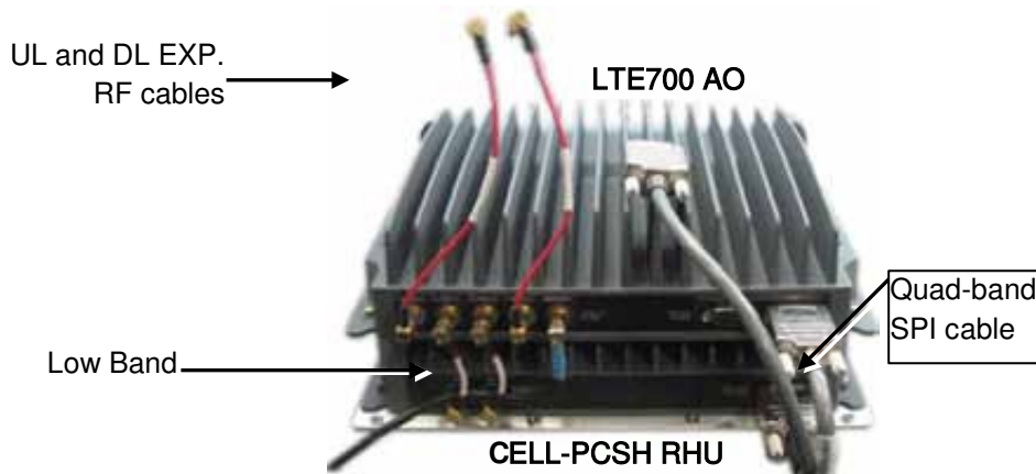
Figure 4-4. RHU and AO Units
