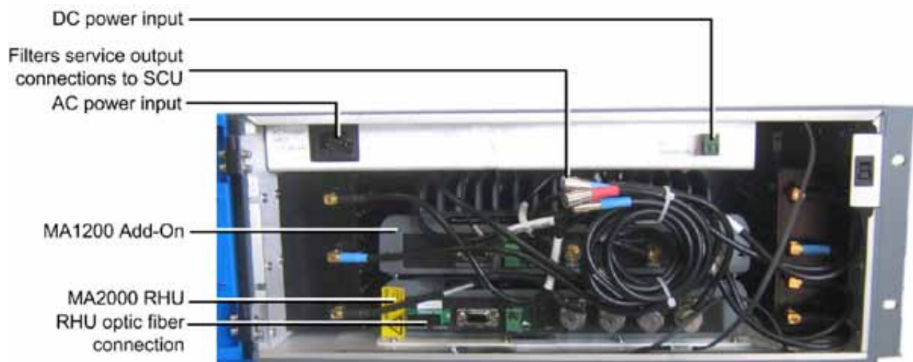
Figure 2-2. MA2000 TSX Open Cabinet View
