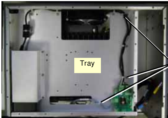
Figure 4-1. Top View of Tray Connections
