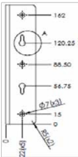
Figure 3-6. Front View of Brackets
