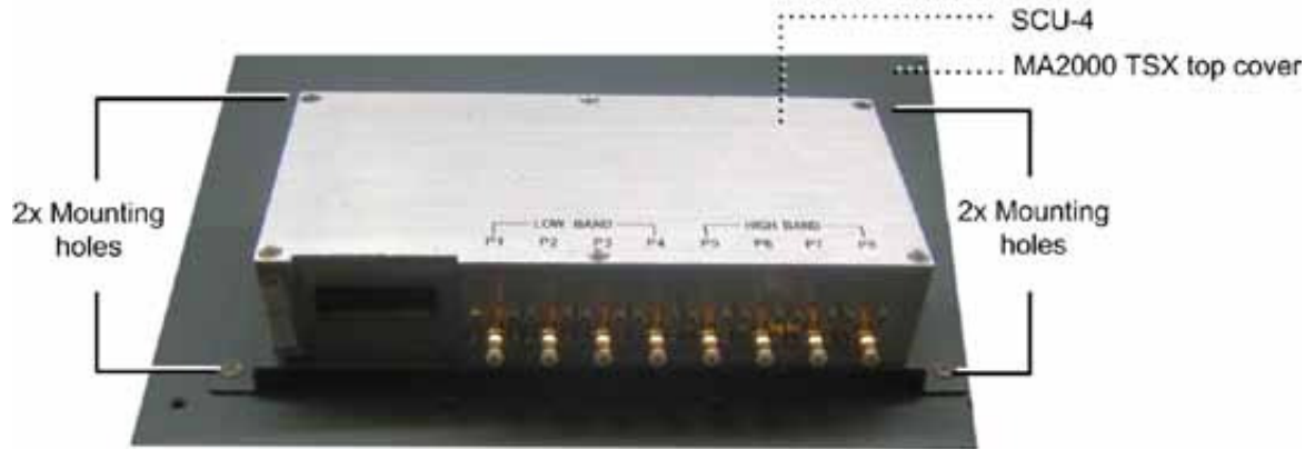
Figure 3-2. SCU-4 Mounted on TSX Unit
