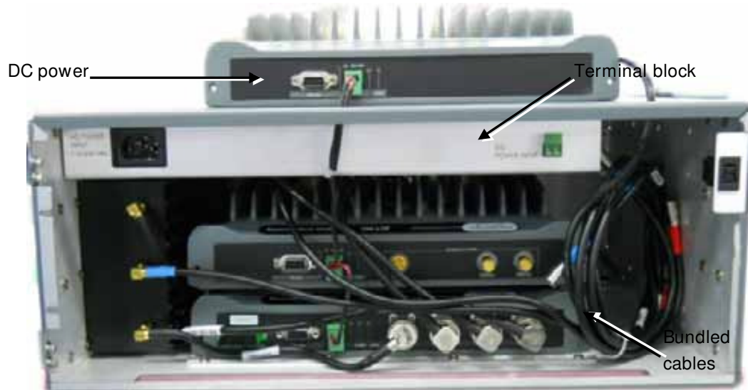
Figure 4-10. Power Connections
