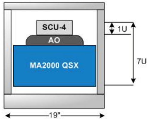
Figure 3-3. Basic MA2000 QSX with SCU-4 Rack Installation Diagram
