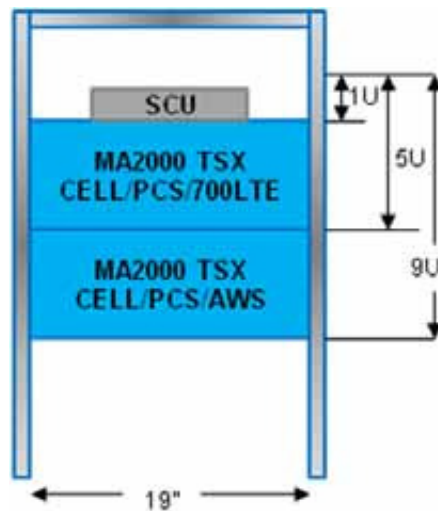
Figure 3-1. Basic MA2000 TSX with SCU-4 Rack Installation Diagram
