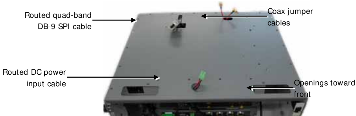
Figure 4-6. TSX Top Cover Openings
