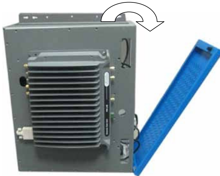
Figure 3-15. Front View of MA2000 QSX Mounted Vertically on Wall
