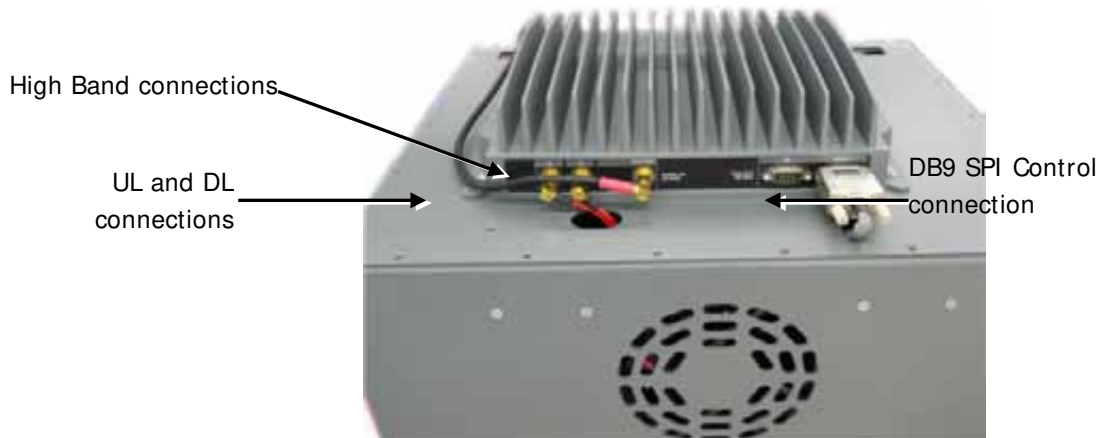
Figure 4-9: AWS AO Rear Panel Cable Connections
