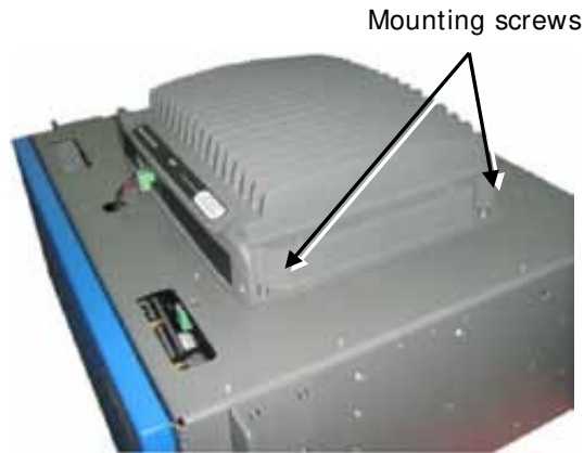
Figure 4-8. AO Unit Mounting Holes – General Location
