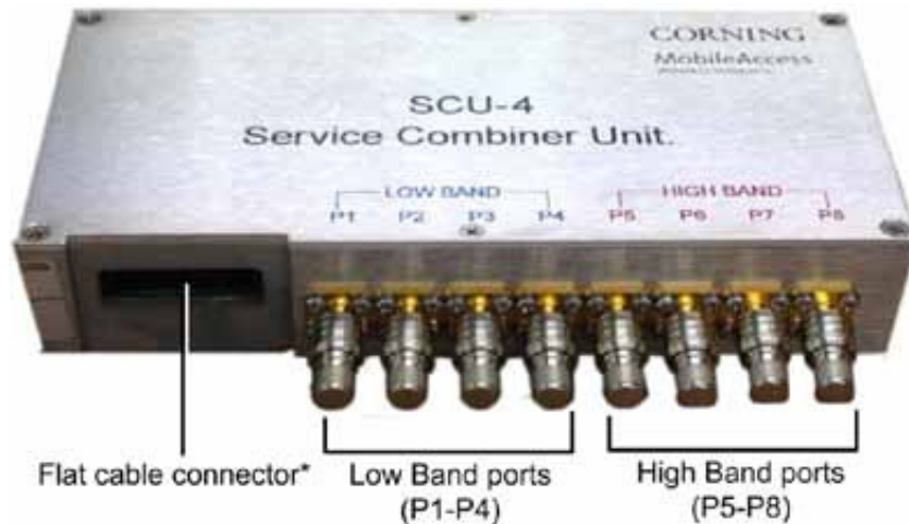
Figure 2-4. SCU-4 (Front Panel)
