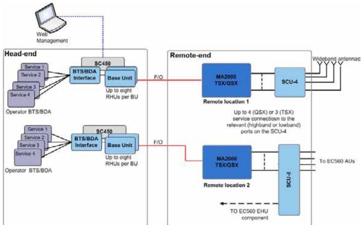
Figure 2-1. MA2000 TSX/QSX Architecture Diagram
