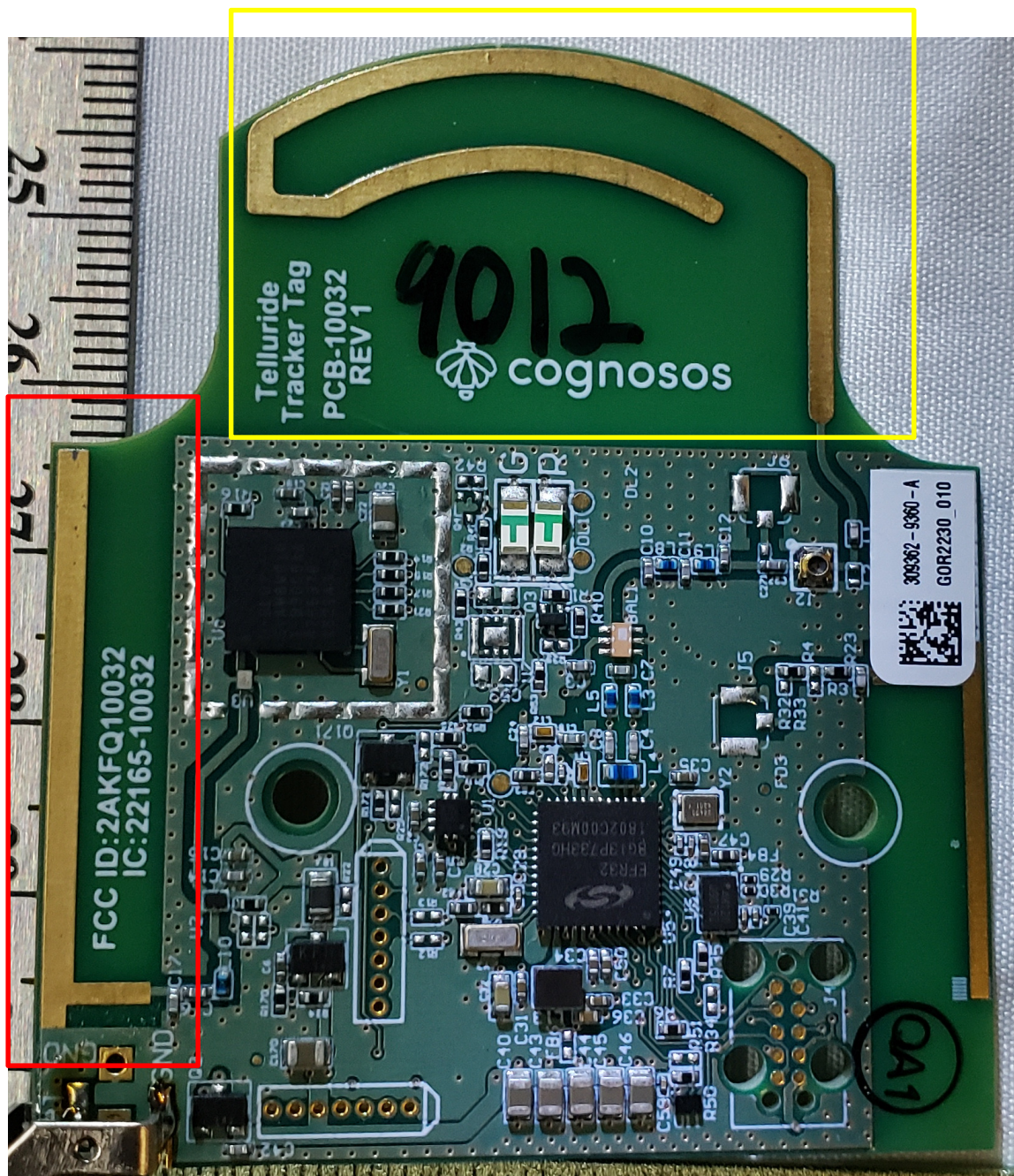
Figure 1. Radio Circuit
