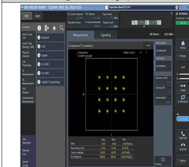
1-N7-PC3-15-40-M-7-CP-16QAM-Outer_Full-216@0-Ant1-see graph-PASS
