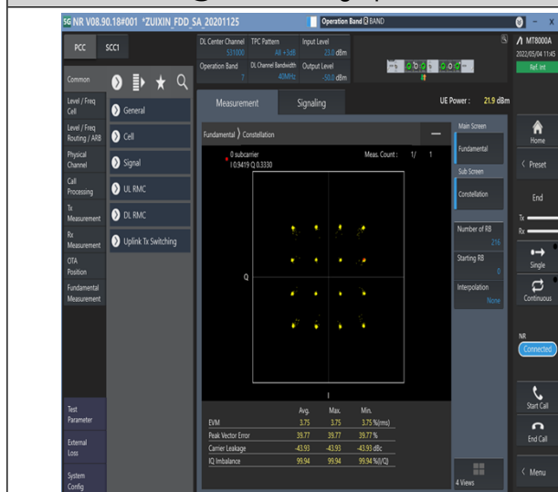
1-N7-PC3-15-40-M-3-DFT-16QAM-Outter_Full-216@0-Ant1-see graph-PASS
