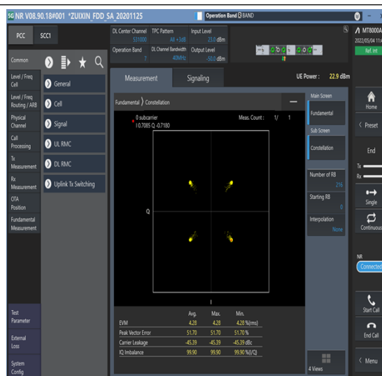
1-N7-PC3-15-40-M-2-DFT-QPSK-Outter_Full-216@0-Ant1-see graph-PASS
