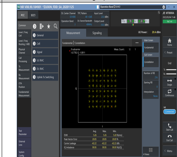
1-N7-PC3-15-40-M-8-CP-64QAM-Outer_Full-216@0-Ant1-see graph-PASS
