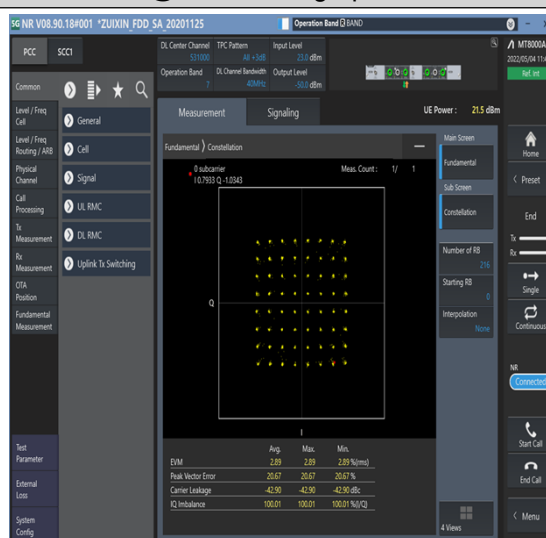
1-N7-PC3-15-40-M-4-DFT-64QAM-Outter_Full-216@0-Ant1-see graph-PASS
