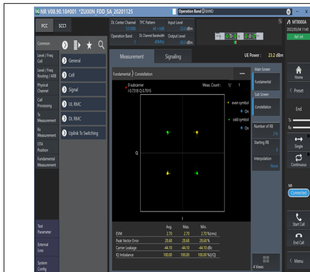
1-N7-PC3-15-40-M-1-DFT-PI2BPSK-Outter_Full-216@0-Ant1-see graph-PASS
