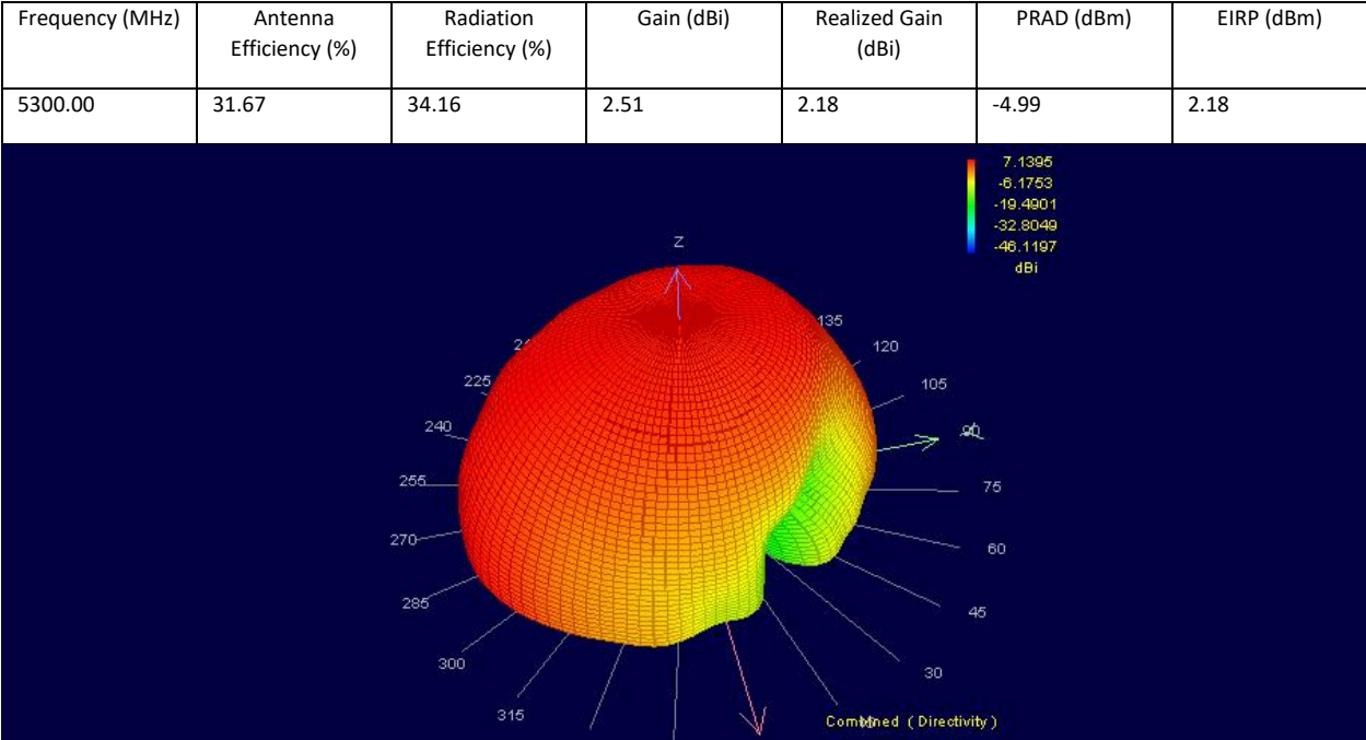
Figure 23 : 3D Far-Field Combined
