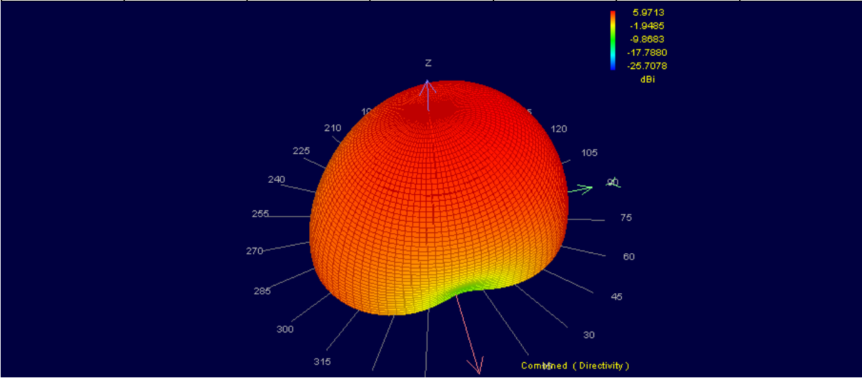
Figure 8 : 3D Far-Field Combined
