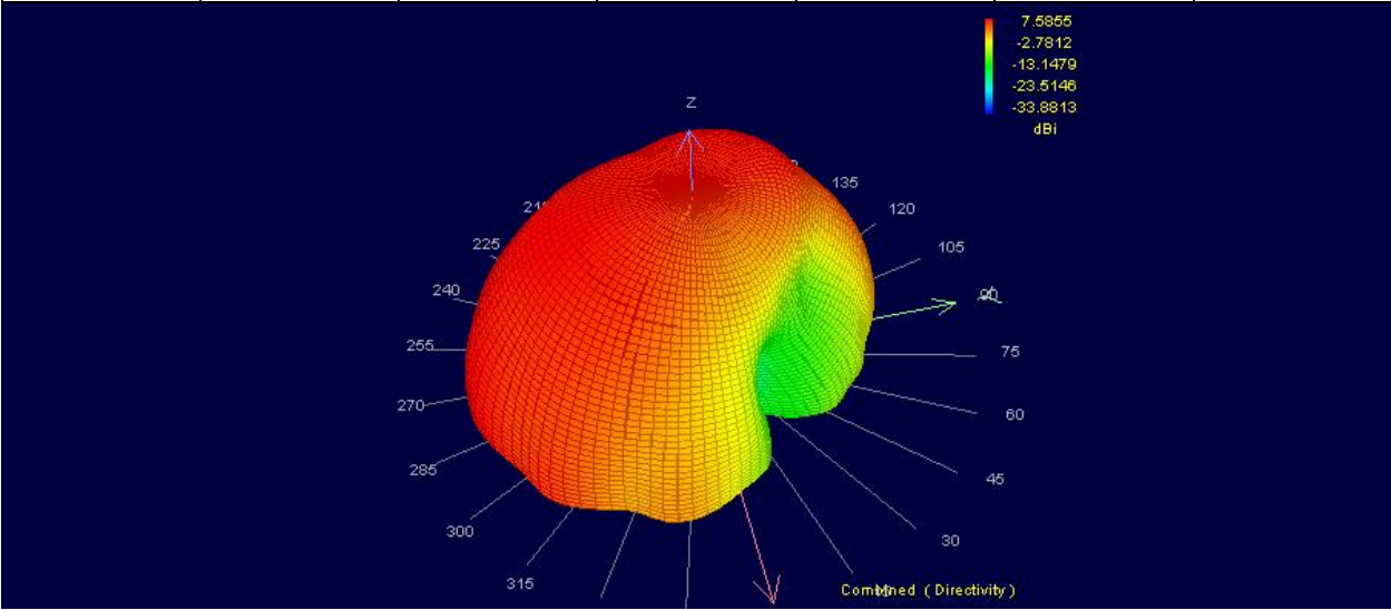
Figure 27 : 3D Far-Field Combined
