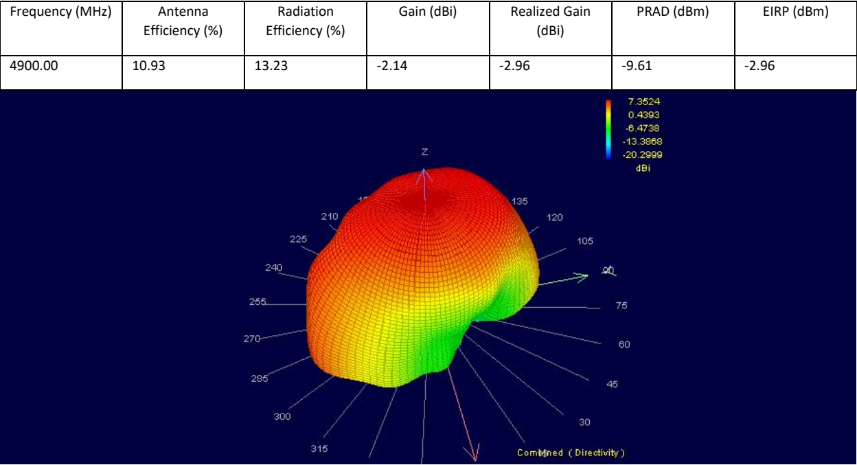
Figure 19 : 3D Far-Field Combined
