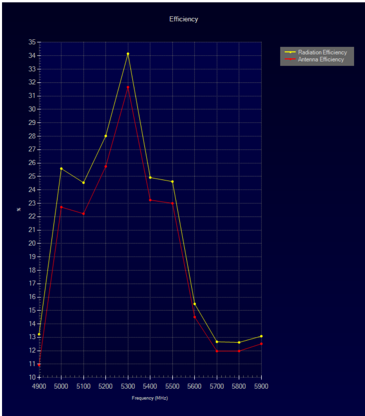
Figure 17 : Efficiency Chart
