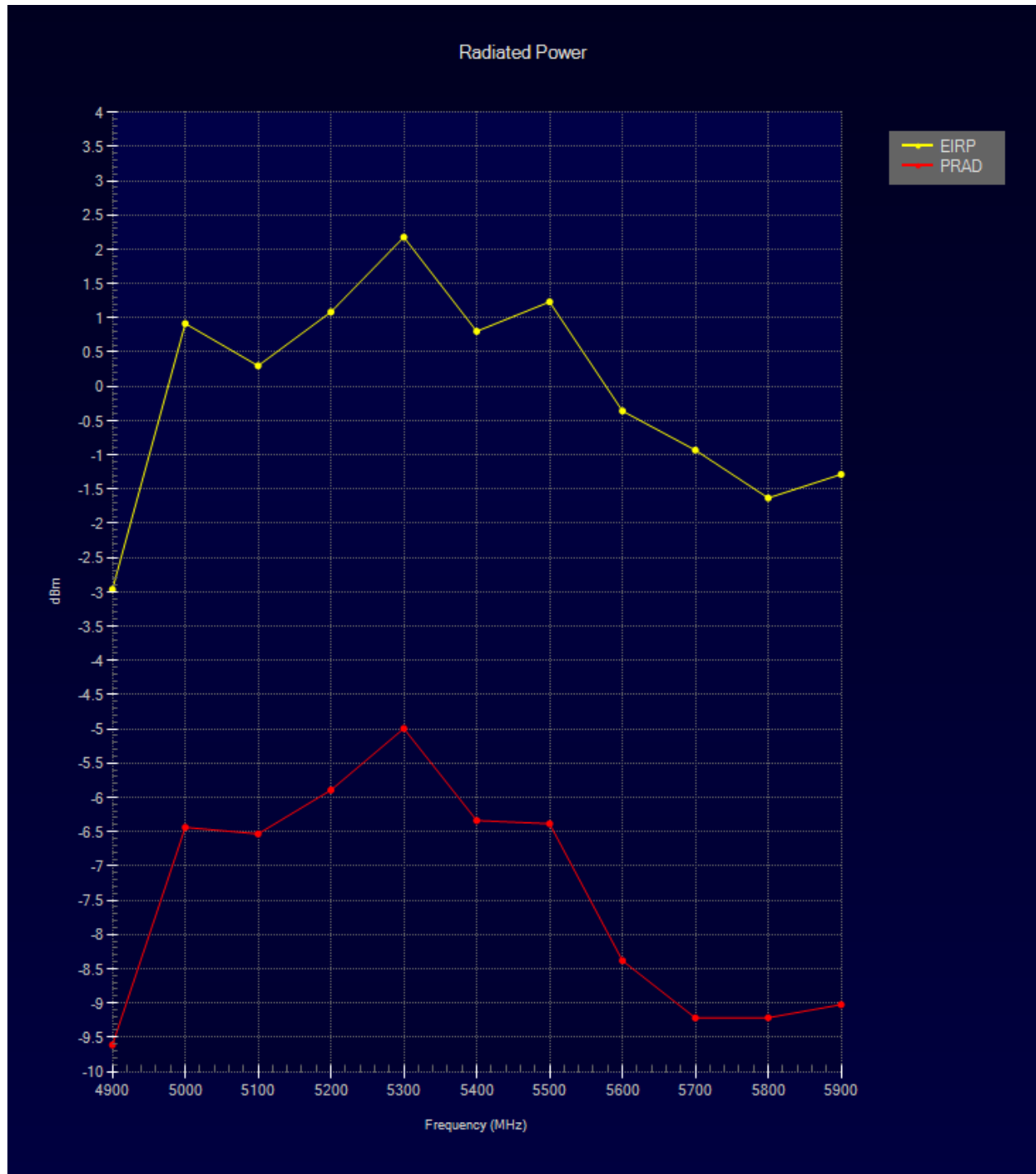
Figure 15 : Radiated Power Chart
