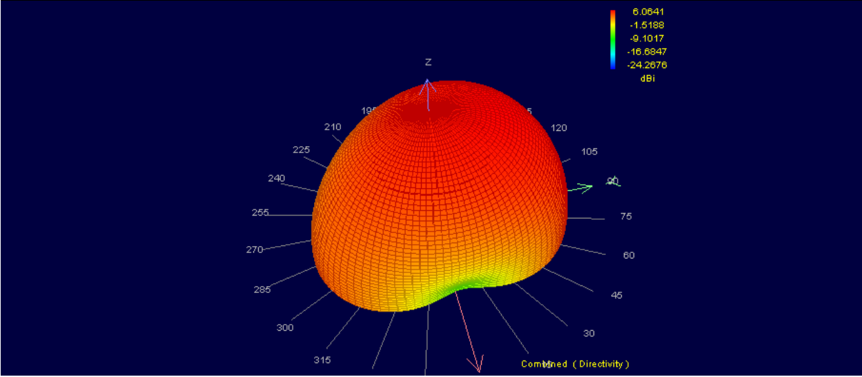
Figure 9 : 3D Far-Field Combined
