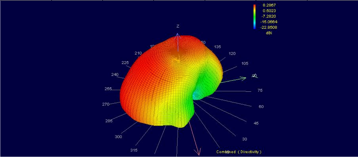
Figure 26 : 3D Far-Field Combined
