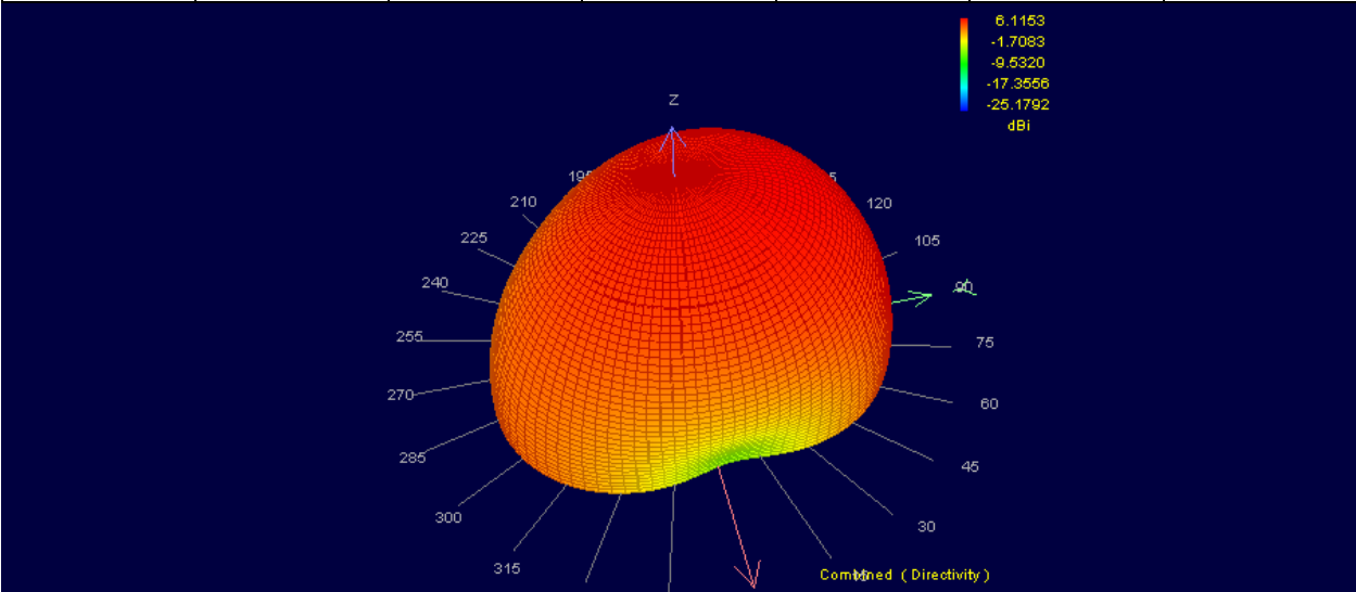
Figure 11 : 3D Far-Field Combined
