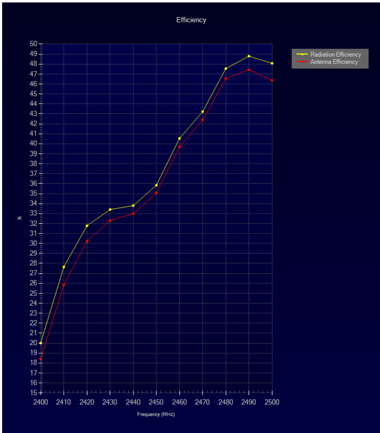
Figure 3 : Efficiency Chart
