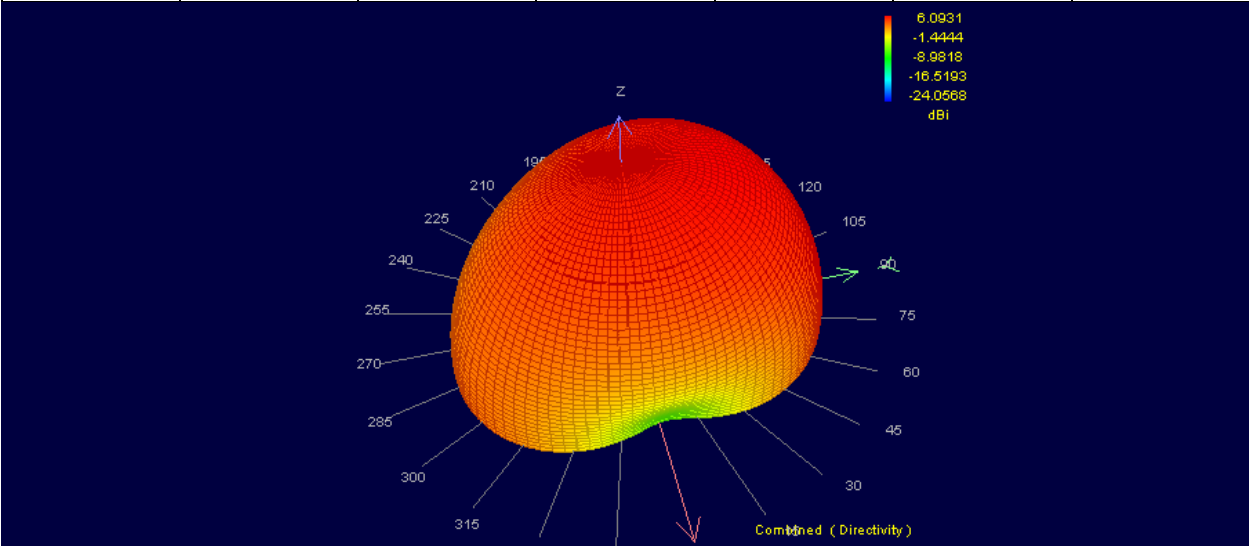
Figure 10 : 3D Far-Field Combined
