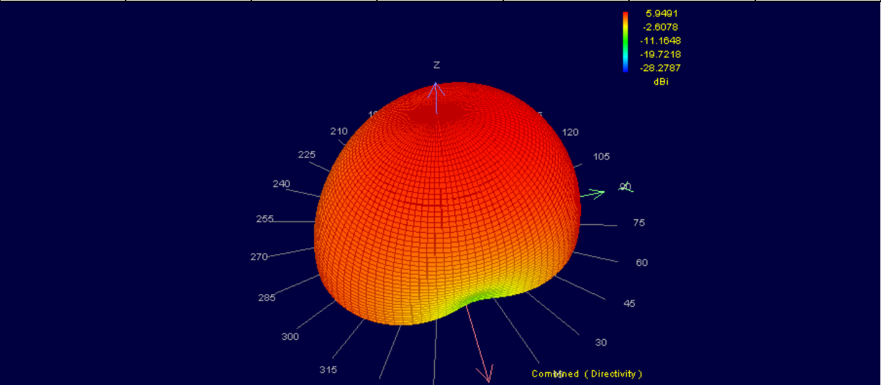
Figure 7 : 3D Far-Field Combined
