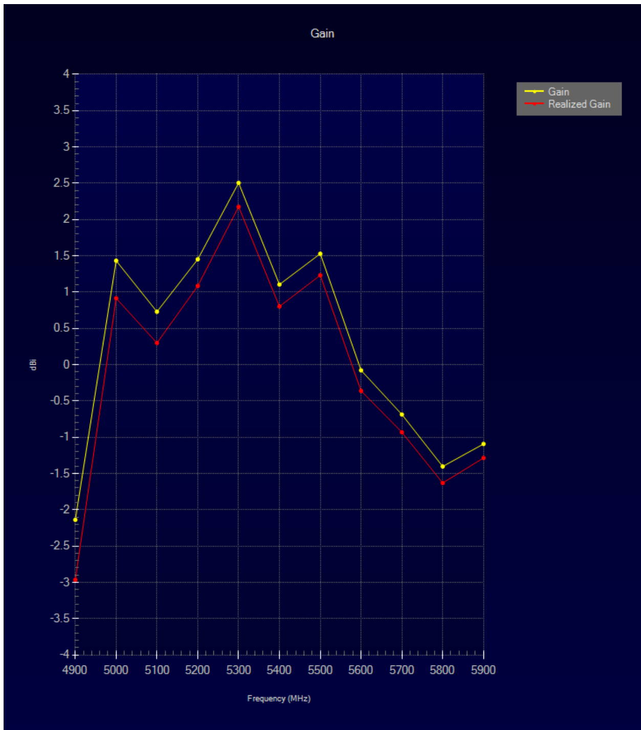
Figure 16 : Gain Chart
