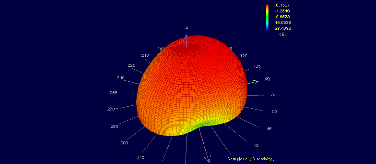
Figure 13 : 3D Far-Field Combined
