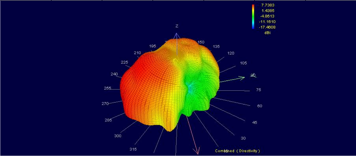
Figure 28 : 3D Far-Field Combined
