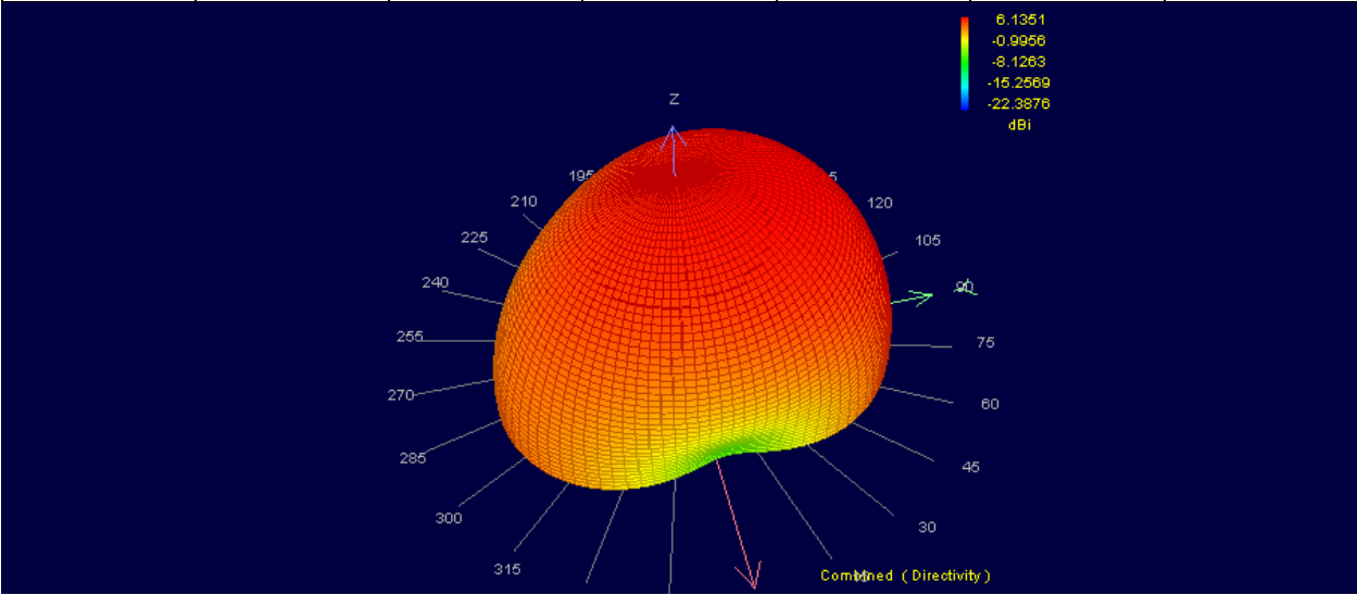
Figure 12 : 3D Far-Field Combined
