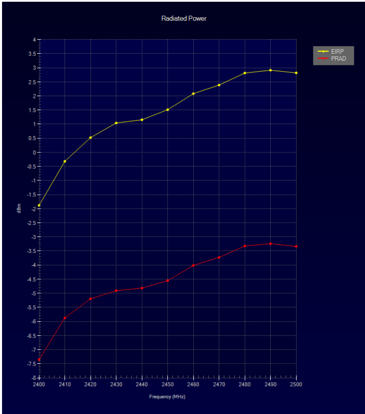
Figure 1 : Radiated Power Chart
