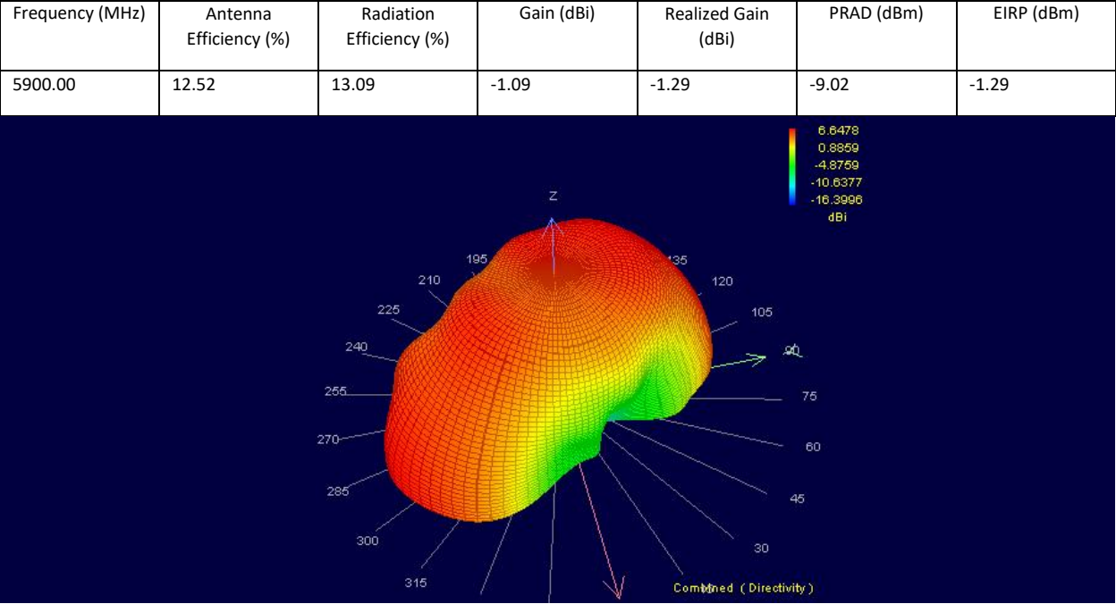
Figure 18 : 3D Far-Field Combined
