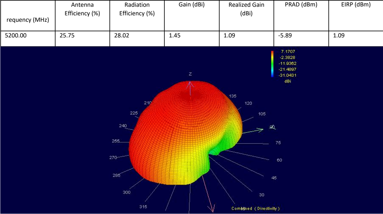
Figure 22 : 3D Far-Field Combined
