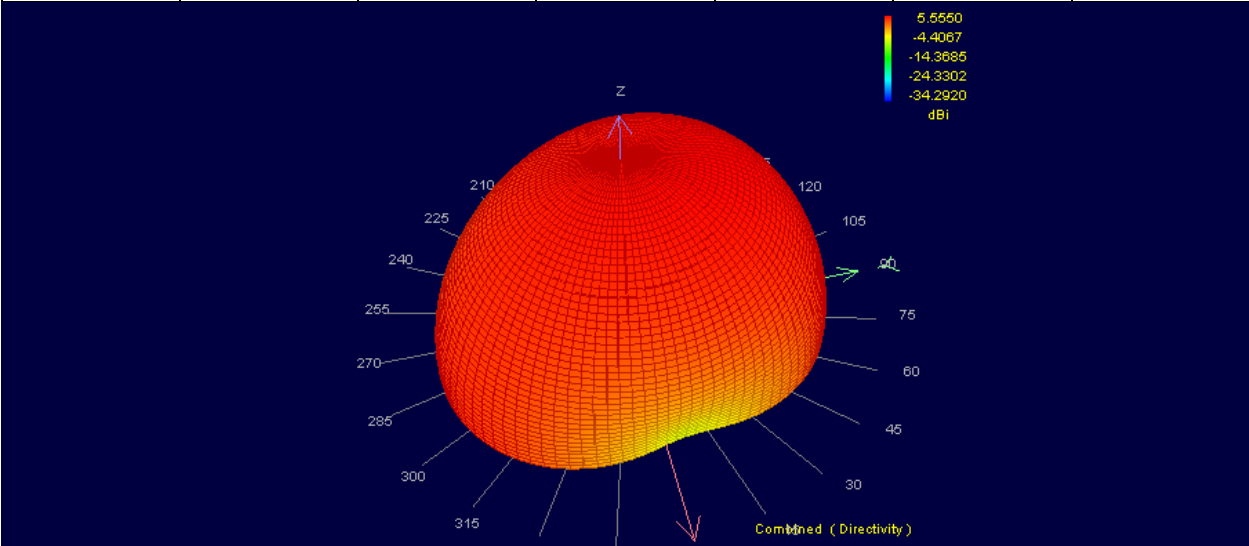
Figure 5 : 3D Far-Field Combined
