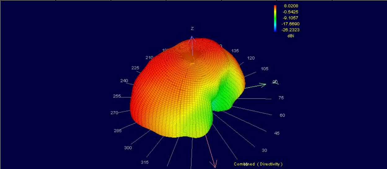
Figure 25 : 3D Far-Field Combined
