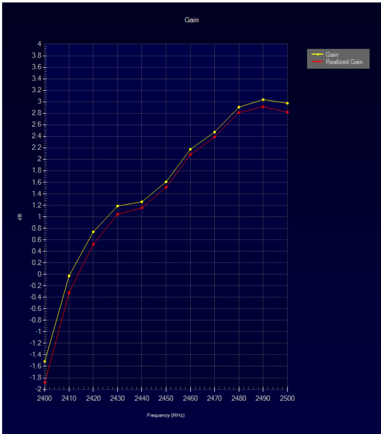
Figure 2 : Gain Chart
