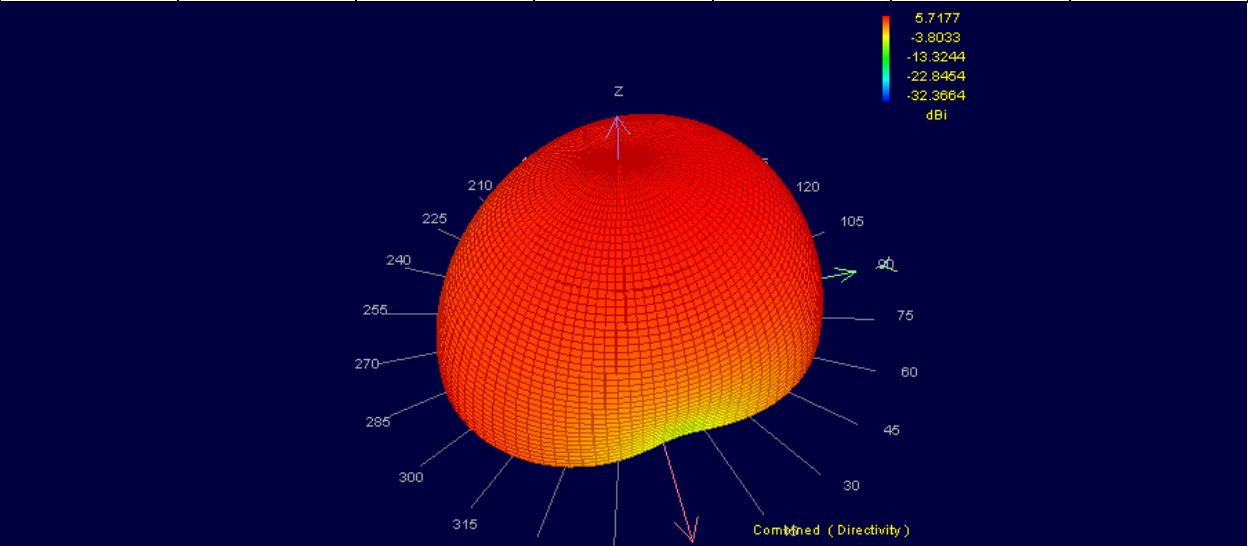
Figure 6 : 3D Far-Field Combined
