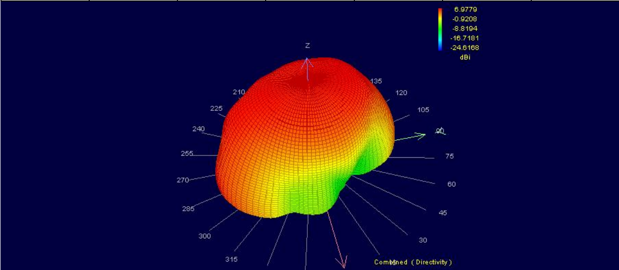
Figure 21 : 3D Far-Field Combined
