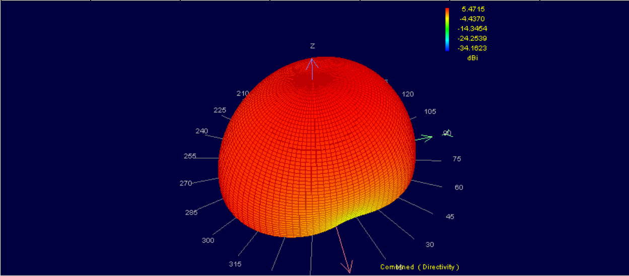
Figure 4 : 3D Far-Field Combined
