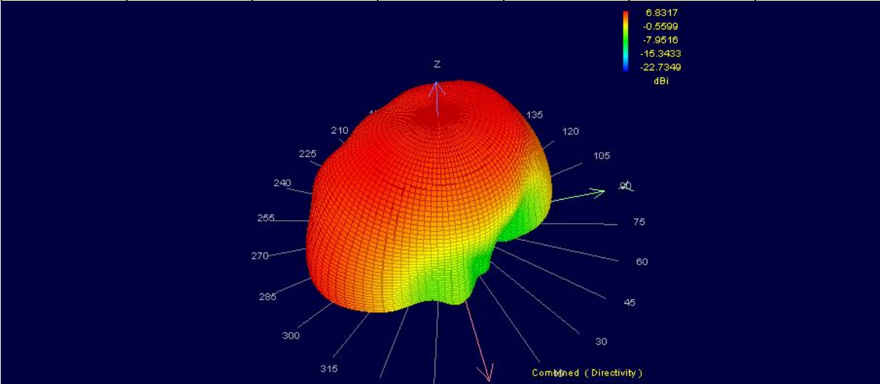
Figure 20 : 3D Far-Field Combined
