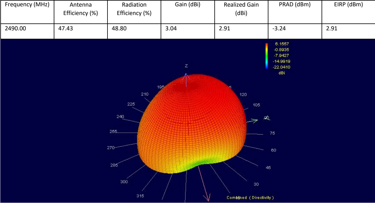
Figure 14 : 3D Far-Field Combined
