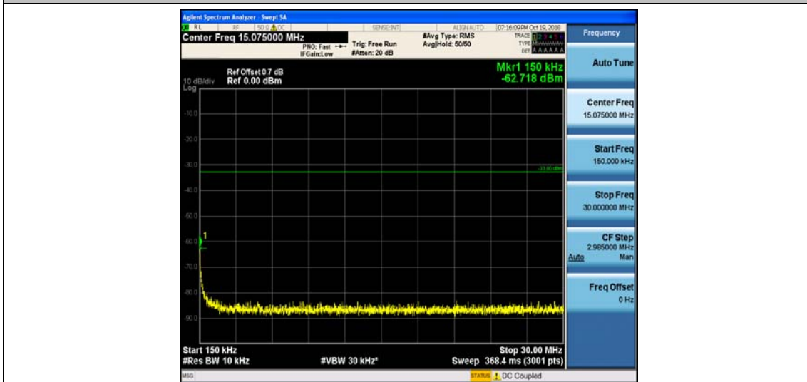
Band4_15MHz_16QAM_20025_1RB#0
