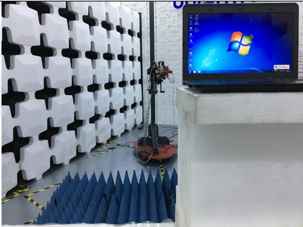
Radiated emission Test Setup (Above 1 GHz) -Dongle
