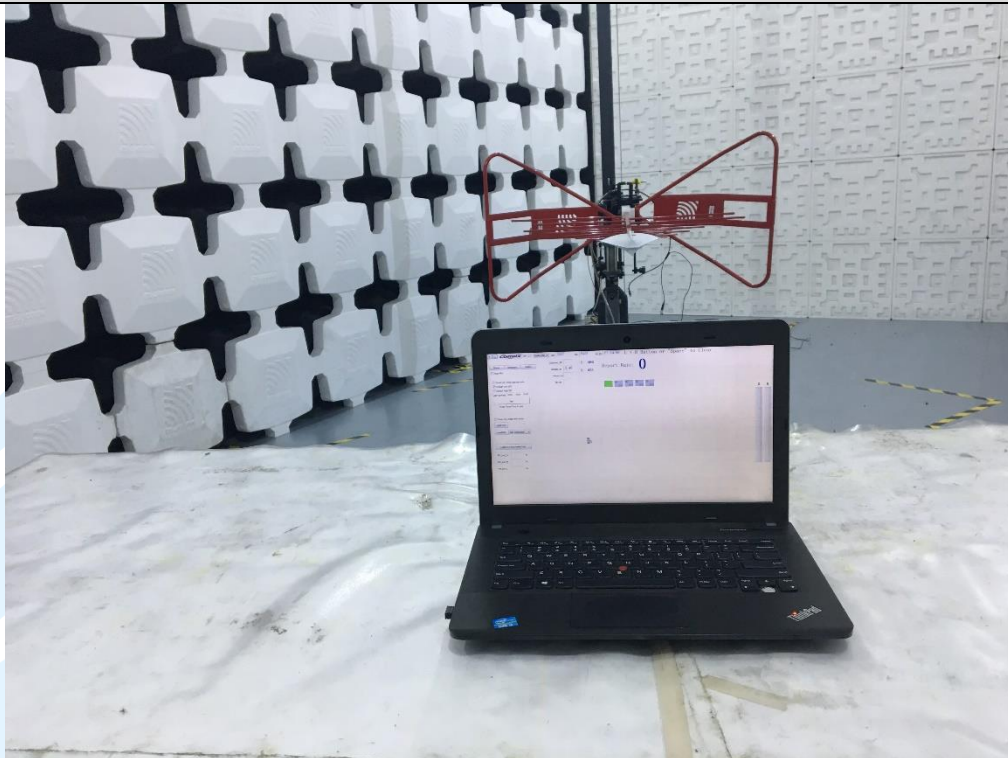
Radiated emission Test Setup (30 MHz~1 GHz)-Dongle
