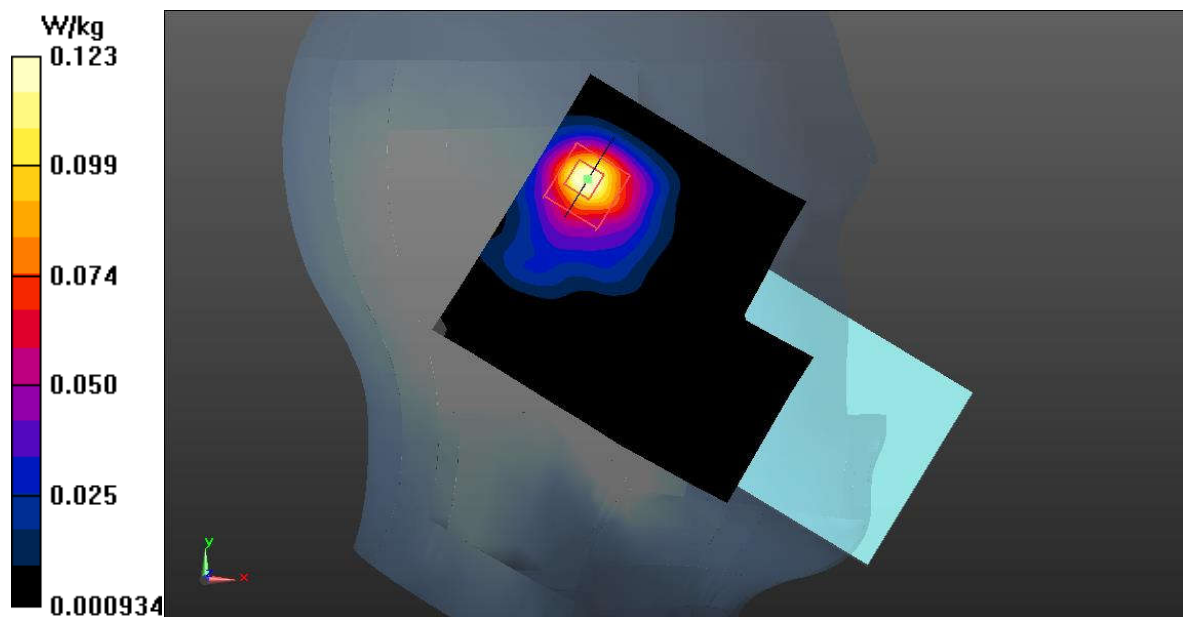
Fig.27 Bluetooth Head
