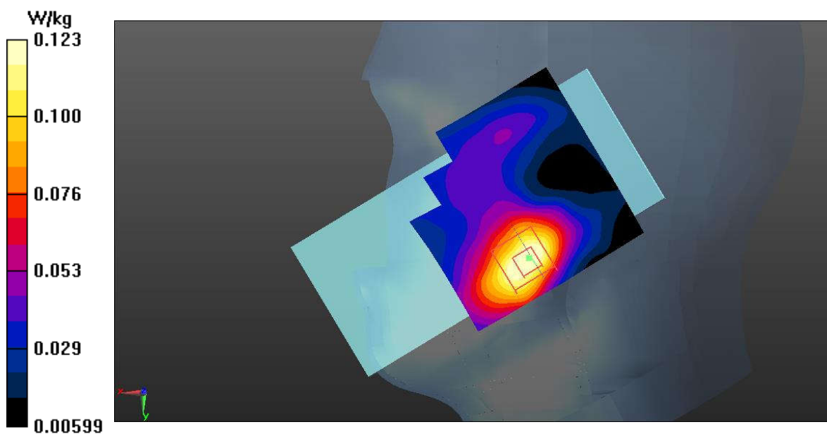
Fig.3 GSM1900 Head
