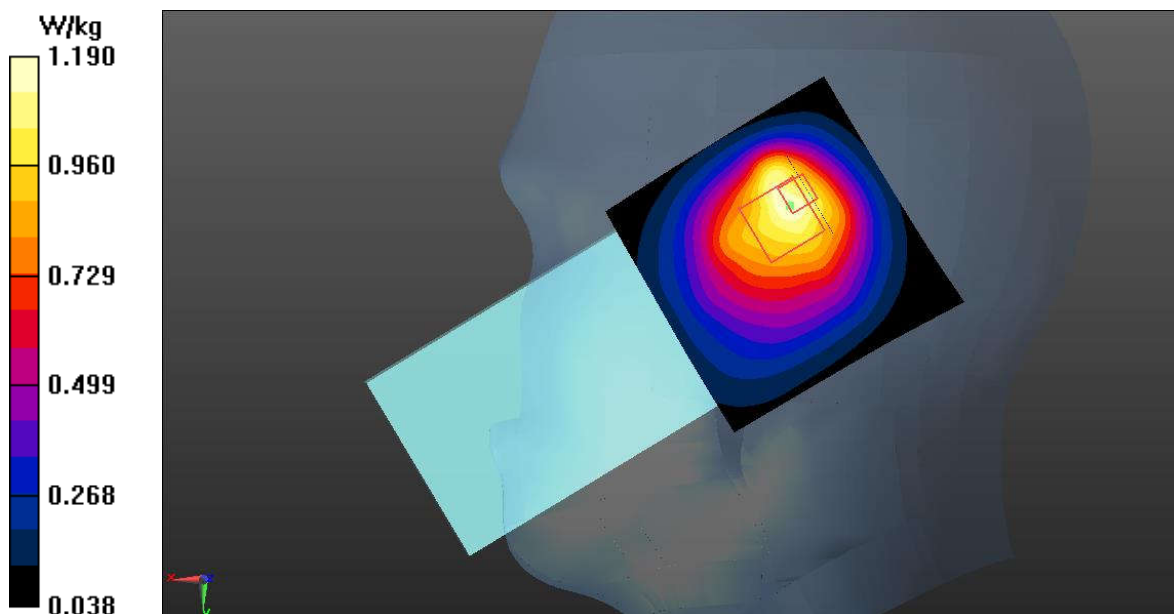
Fig.1 GSM850 Head
