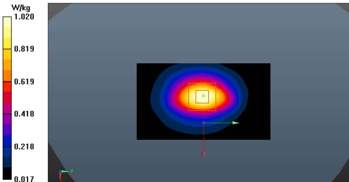
Fig.4 GSM1900 Body
