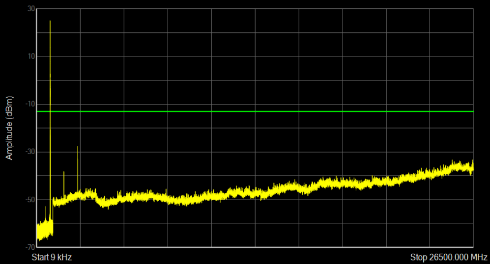
Band26(824-849) QPSK BW=3MHz Channel=26915 RB Size=1 Position=#0
