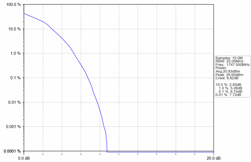
Band4_15MHz_16QAM_HCH_1747.5MHz_RB_27_48_NTNV
