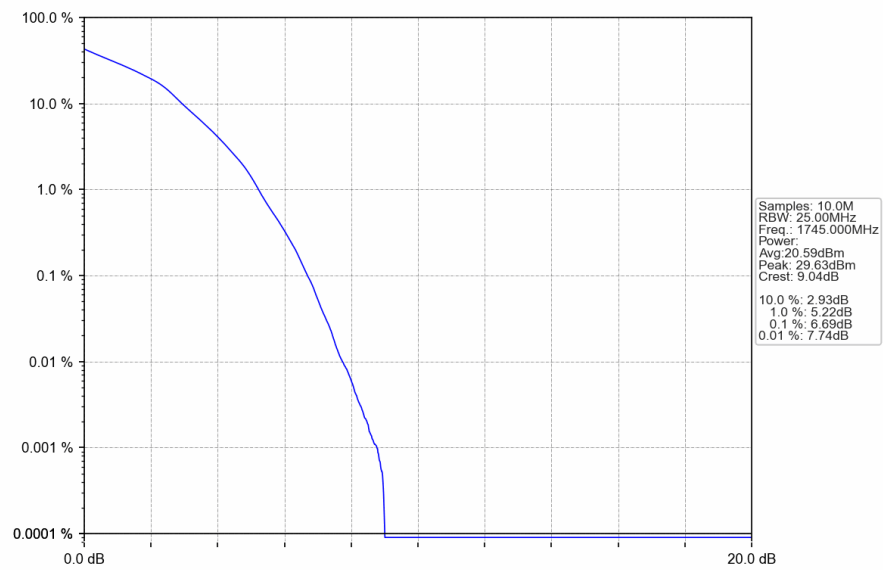
Band4 20MHz 16QAM HCH 1745MHz RB 27 73 NTN
