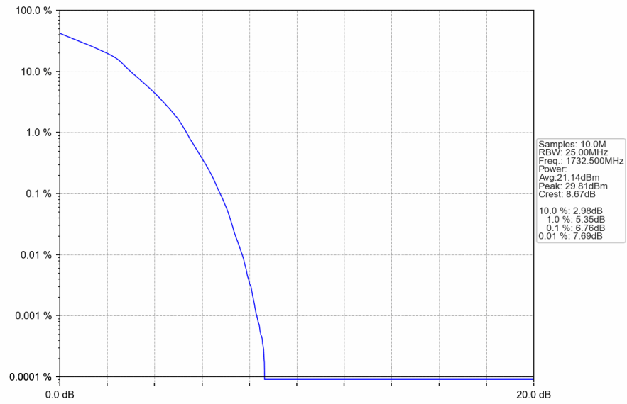
Band4_15MHz_16QAM_MCH_1732.5MHz_RB_27_0_NTNV
