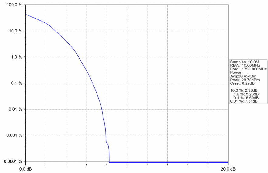
Band4_10MHz_16QAM_HCH_1750MHz_RB_27_23_NTNV
