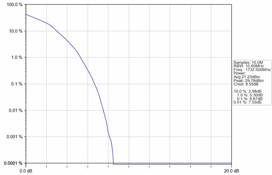
Band4_10MHz_16QAM_MCH_1732.5MHz_RB_27_0_NTNV
