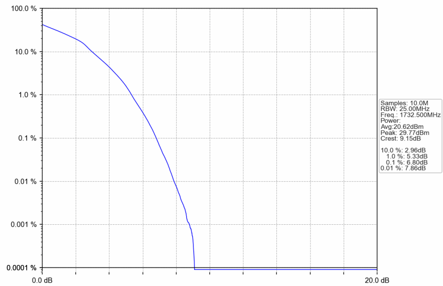
Band4 20MHz 16QAM MCH 1732.5MHz RB 27 0 NTN
