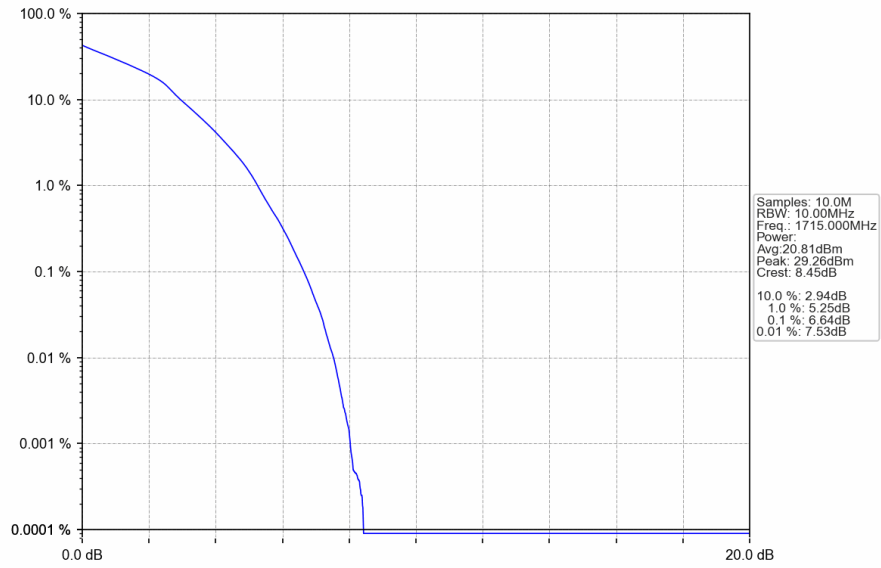
Band4 10MHz 16QAM LCH 1715MHz RB 27 0 NTNV
