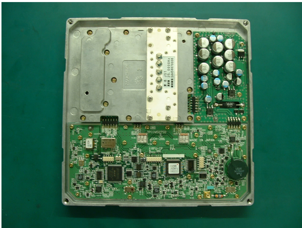
TypeW AP-RFU Internal View
