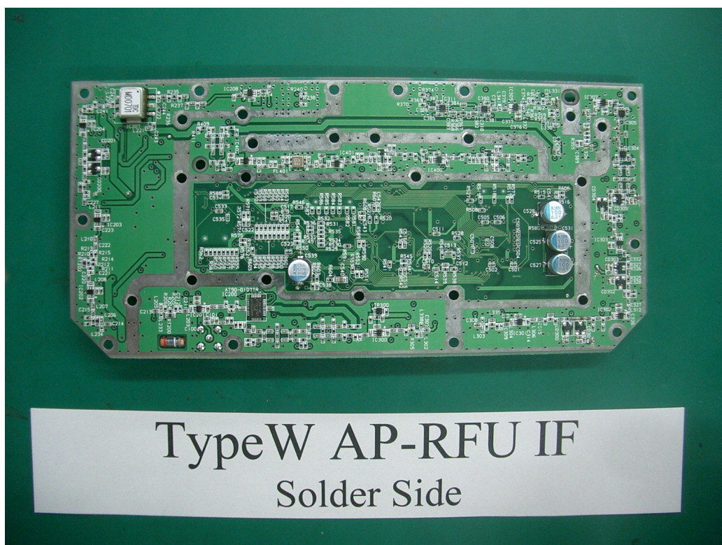
TypeW AP-RFU IF Solder Side Internal View
