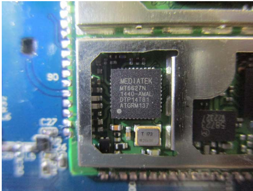
EUT – Bluetooth & WiFi Chip View
