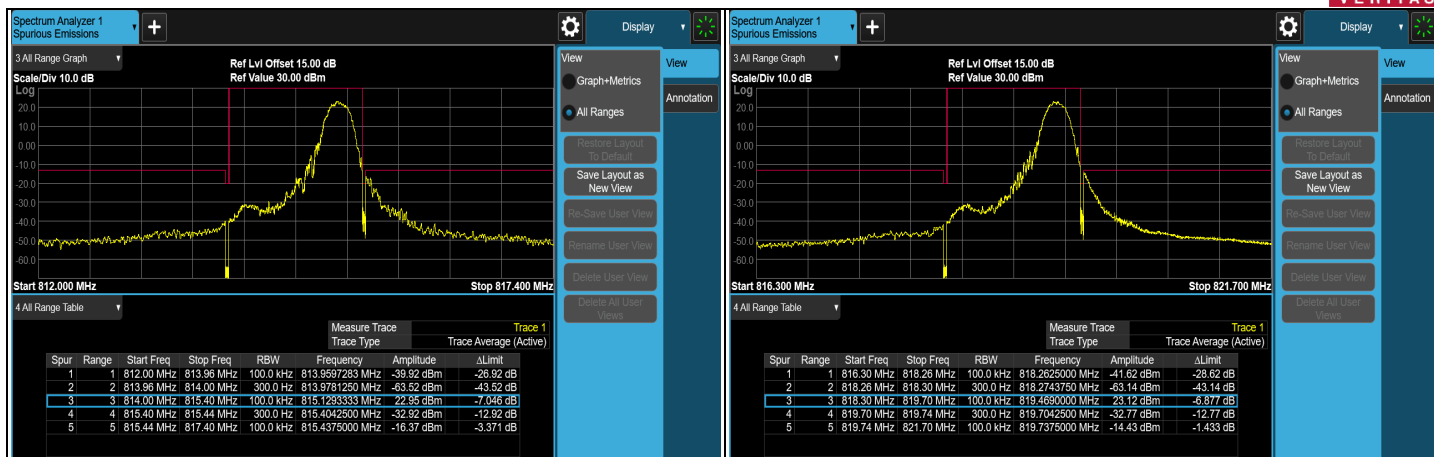
1RB#MAX CH 26697 (814.7 MHz)
