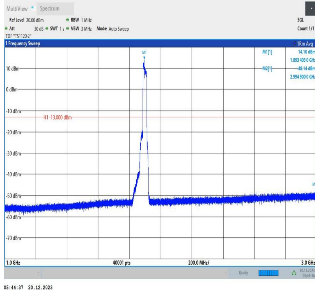
2-2-10MHz-15MHz-QPSK-QPSK-19005-19125-50RB#0-75RB #0-1000~3000MHz-PASS
