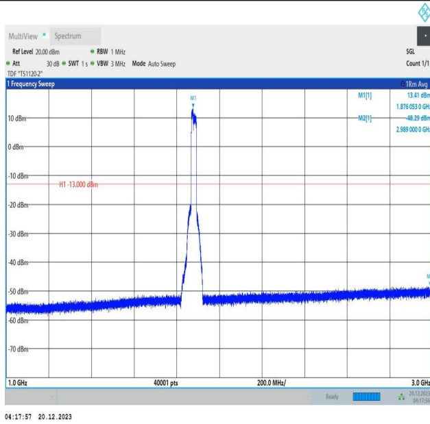
2-2-10MHz-15MHz-QPSK-QPSK-18829-18949-50RB#0-75RB #0-1000~3000MHz-PASS
