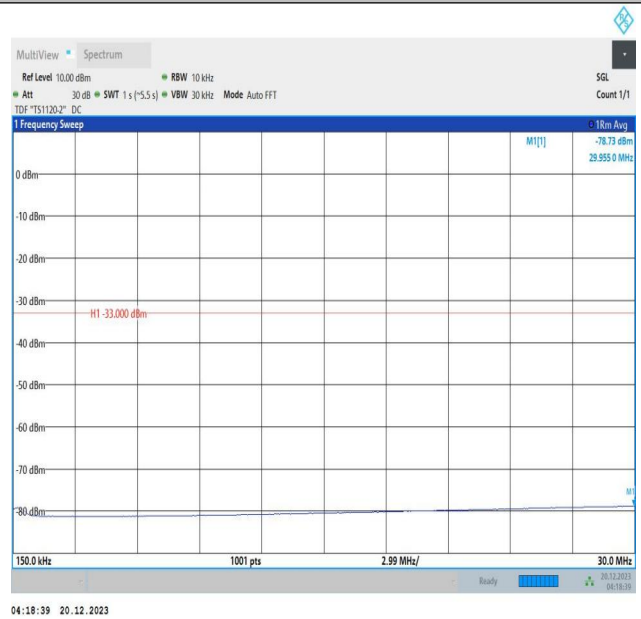
2-2-10MHz-15MHz-16QAM-16QAM-18829-18949-50RB#0-75 RB#0-0.15~30MHz-PASS
