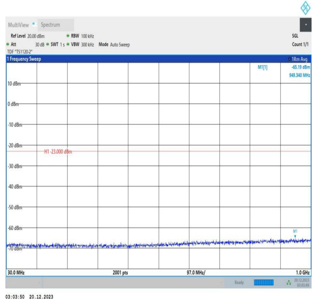
2-2-10MHz-15MHz-16QAM-16QAM-18829-18949-1RB#0-0RB #0-30~1000MHz-PASS
