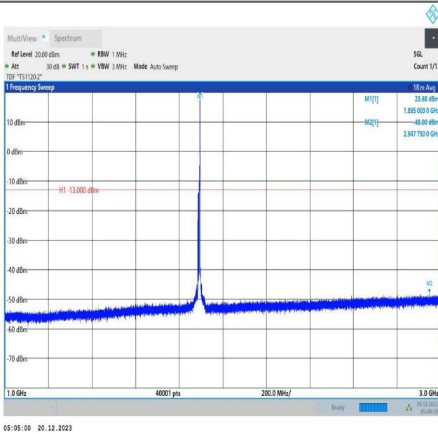
2-2-10MHz-15MHz-QPSK-QPSK-19005-19125-1RB#49-0RB# 0-1000~3000MHz-PASS
