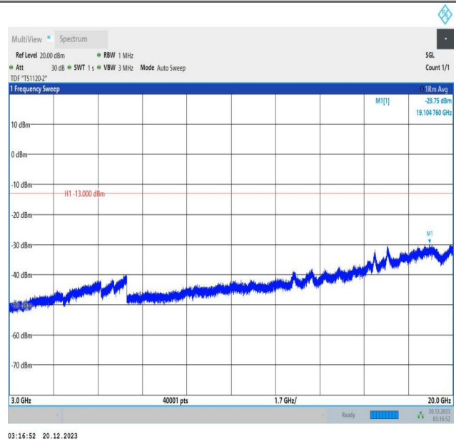
2-2-10MHz-15MHz-QPSK-QPSK-18829-18949-1RB#49-0RB# 0-3000~20000MHz-PASS
