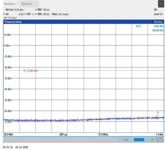
2-2-10MHz-15MHz-64QAM-64QAM-18653-18773-50RB#0-75 RB#0-30~1000MHz-PASS
