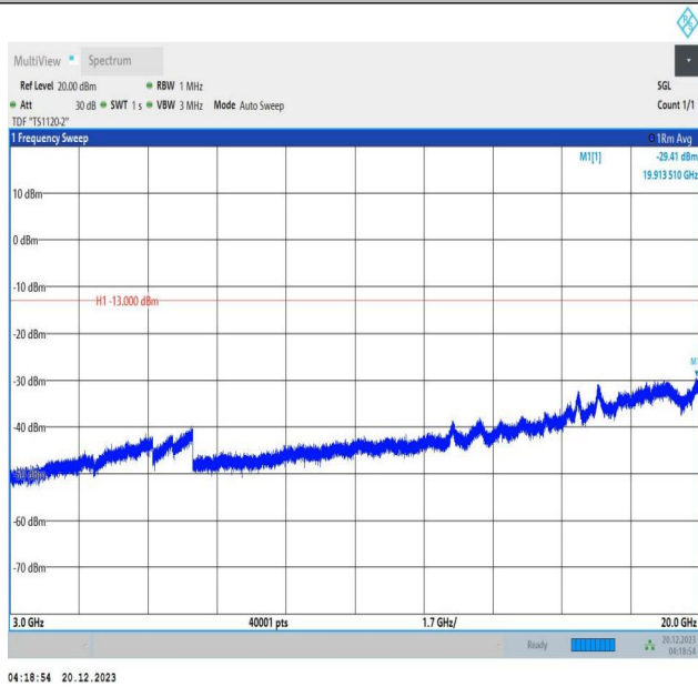
2-2-10MHz-15MHz-16QAM-16QAM-18829-18949-50RB#0-75 RB#0-3000~20000MHz-PASS
