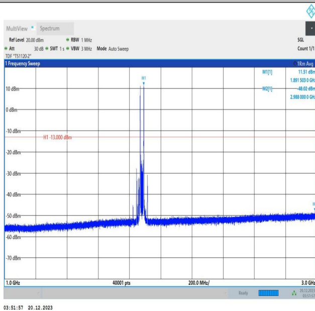
2-2-10MHz-15MHz-16QAM-16QAM-18829-18949-1RB#0-1RB #74-1000~3000MHz-PASS
