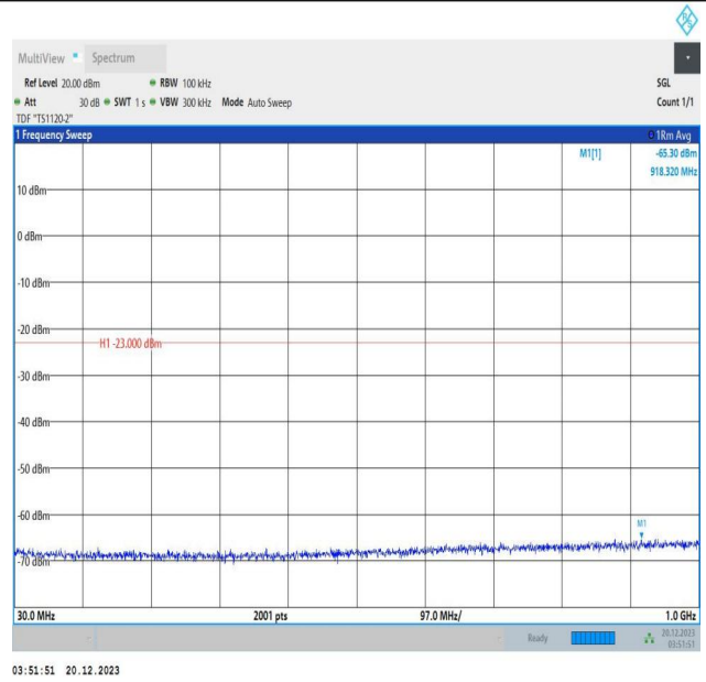
2-2-10MHz-15MHz-16QAM-16QAM-18829-18949-1RB#0-1RB #74-30~1000MHz-PASS
