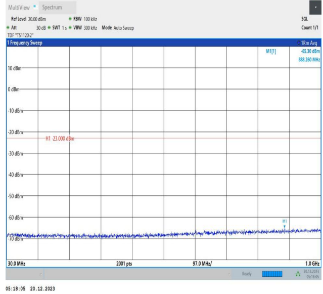
2-2-10MHz-15MHz-16QAM-16QAM-19005-19125-1RB#0-1RB #74-30~1000MHz-PASS
