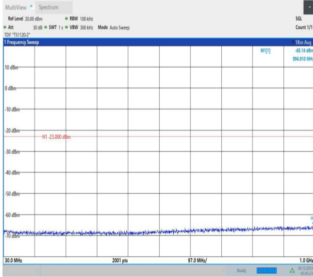
2-2-10MHz-15MHz-16QAM-16QAM-19005-19125-50RB#0-75 RB#0-30~1000MHz-PASS
