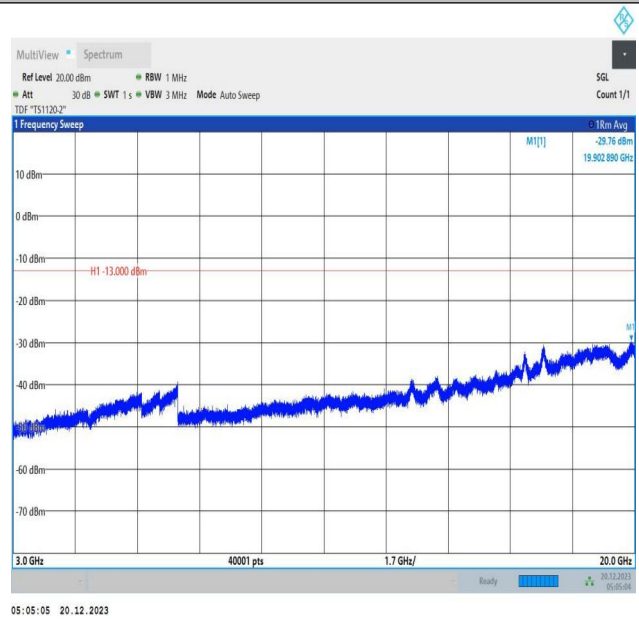
2-2-10MHz-15MHz-QPSK-QPSK-19005-19125-1RB#49-0RB# 0-3000~20000MHz-PASS
