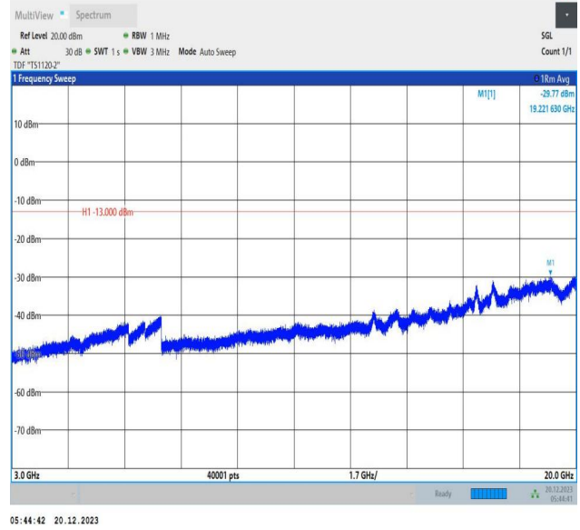
2-2-10MHz-15MHz-QPSK-QPSK-19005-19125-50RB#0-75RB #0-3000~20000MHz-PASS
