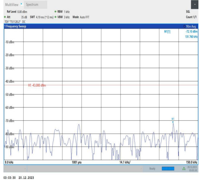
2-2-10MHz-15MHz-16QAM-16QAM-18829-18949-1RB#0-0RB #0-0.009~0.15MHz-PASS
