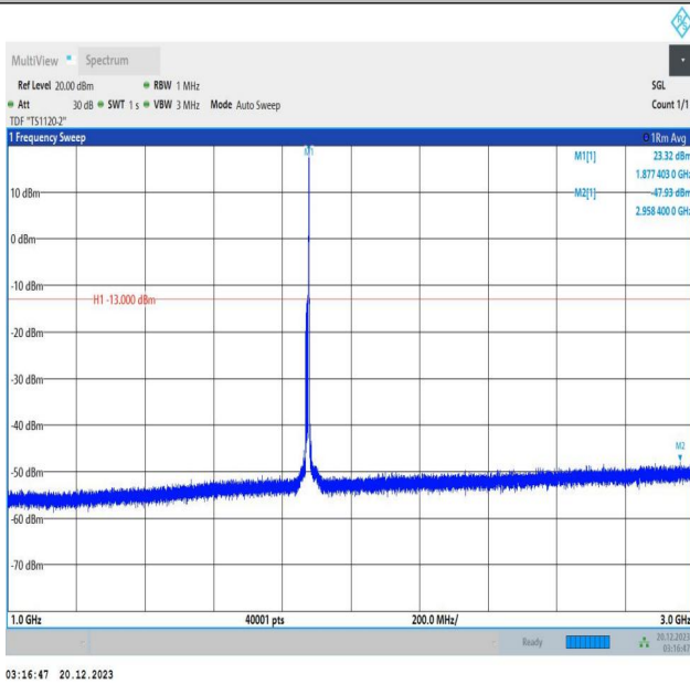
2-2-10MHz-15MHz-QPSK-QPSK-18829-18949-1RB#49-0RB# 0-1000~3000MHz-PASS
