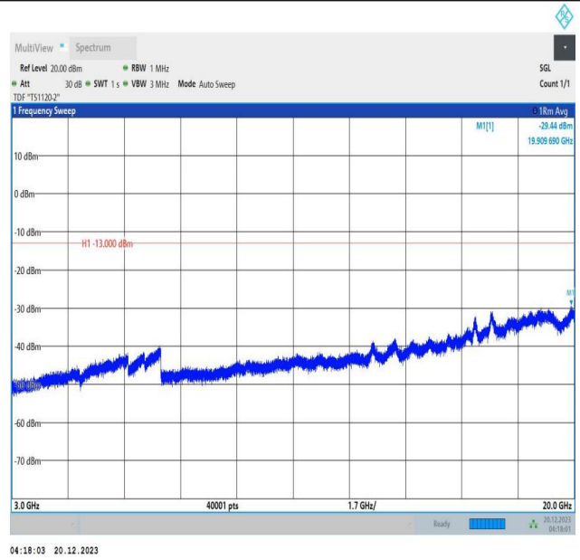
2-2-10MHz-15MHz-QPSK-QPSK-18829-18949-50RB#0-75RB #0-3000~20000MHz-PASS
