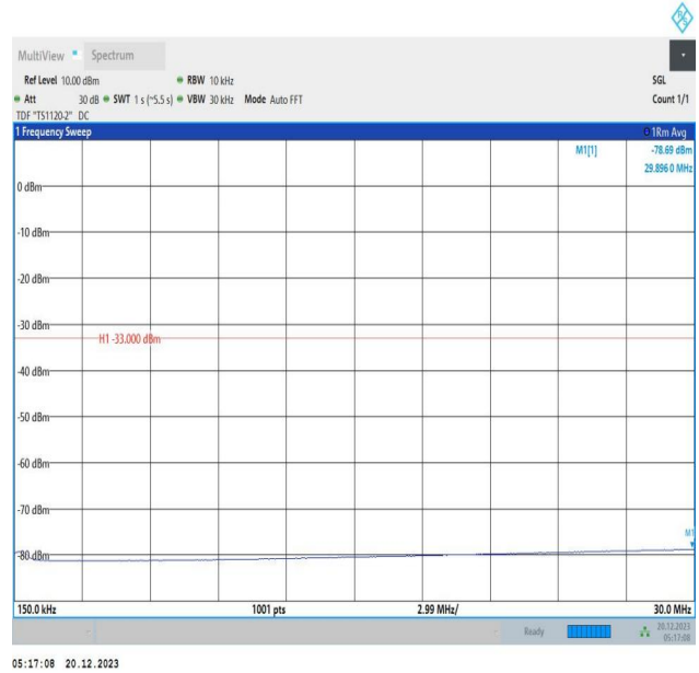
2-2-10MHz-15MHz-QPSK-QPSK-19005-19125-1RB#0-1RB#7 4-0.15~30MHz-PASS
