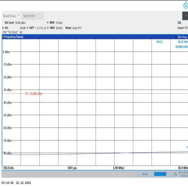
2-2-10MHz-15MHz-QPSK-QPSK-18829-18949-1RB#49-0RB# 0-0.15~30MHz-PASS
