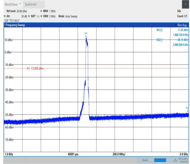
2-2-10MHz-15MHz-16QAM-16QAM-19005-19125-50RB#0-75 RB#0-1000~3000MHz-PASS
