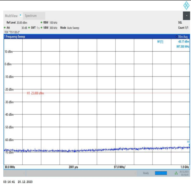
2-2-10MHz-15MHz-QPSK-QPSK-18829-18949-1RB#49-0RB# 0-30~1000MHz-PASS
