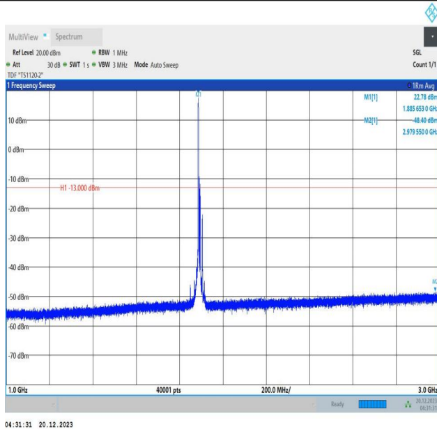
2-2-10MHz-15MHz-16QAM-16QAM-19005-19125-1RB#0-0RB #0-1000~3000MHz-PASS
