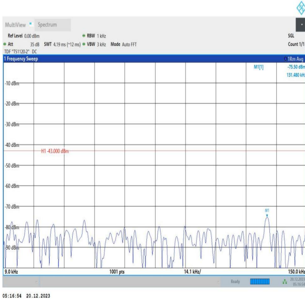
2-2-10MHz-15MHz-QPSK-QPSK-19005-19125-1RB#0-1RB#7 4-0.009~0.15MHz-PASS
