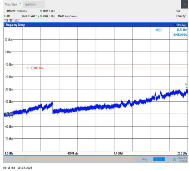
2-2-10MHz-15MHz-64QAM-64QAM-19005-19125-1RB#49-0R B#0-3000~20000MHz-PASS
