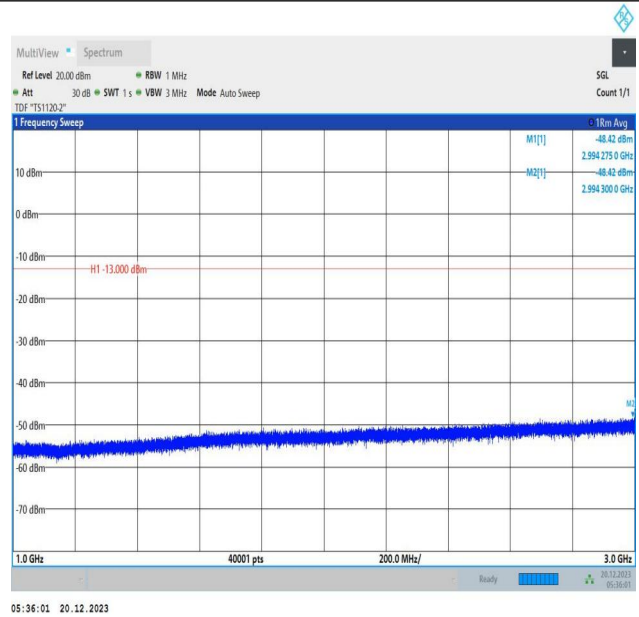
2-2-10MHz-15MHz-64QAM-64QAM-19005-19125-1RB#0-1RB #74-1000~3000MHz-PASS
