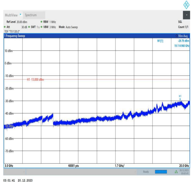
2-2-10MHz-15MHz-64QAM-64QAM-18653-18773-50RB#0-75 RB#0-3000~20000MHz-PASS
