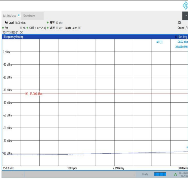
2-2-10MHz-15MHz-64QAM-64QAM-18829-18949-50RB#0-75 RB#0-0.15~30MHz-PASS
