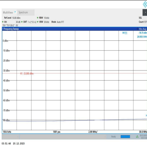
2-2-10MHz-15MHz-16QAM-16QAM-18829-18949-1RB#0-1RB #74-0.15~30MHz-PASS
