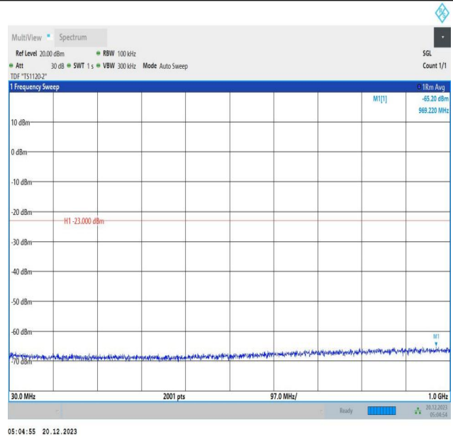
2-2-10MHz-15MHz-QPSK-QPSK-19005-19125-1RB#49-0RB# 0-30~1000MHz-PASS
