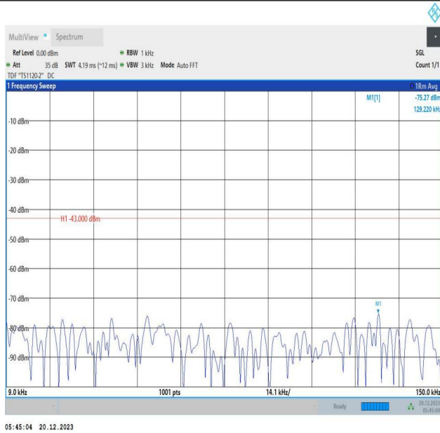
2-2-10MHz-15MHz-16QAM-16QAM-19005-19125-50RB#0-75 RB#0-0.009~0.15MHz-PASS
