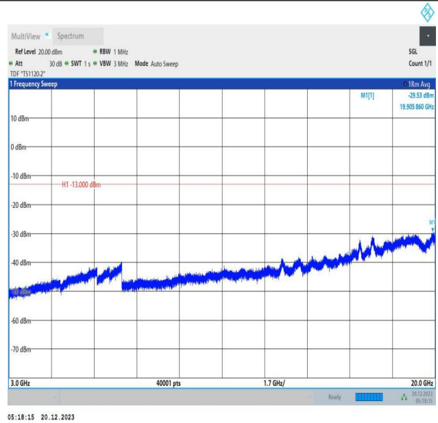
2-2-10MHz-15MHz-16QAM-16QAM-19005-19125-1RB#0-1RB #74-3000~20000MHz-PASS
