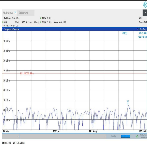
2-2-10MHz-15MHz-64QAM-64QAM-19005-19125-1RB#0-0RB #0-0.009~0.15MHz-PASS
