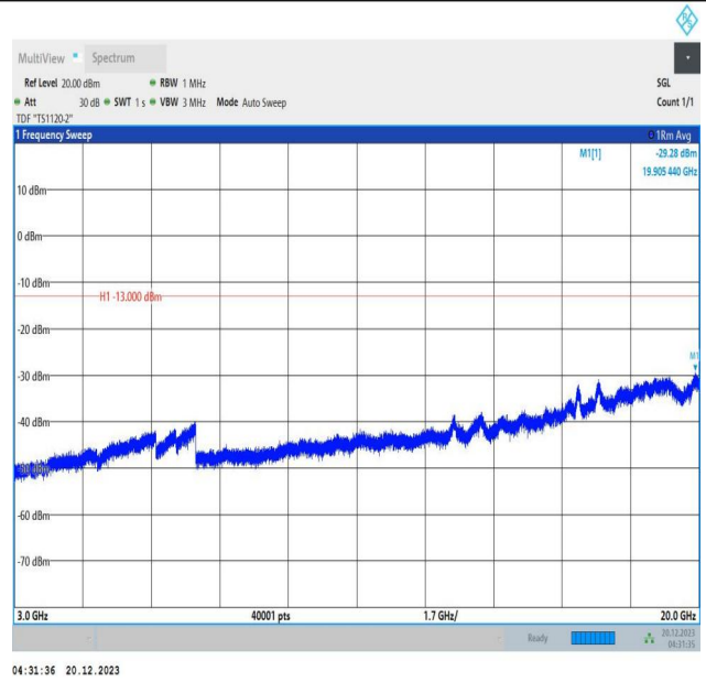
2-2-10MHz-15MHz-16QAM-16QAM-19005-19125-1RB#0-0RB #0-3000~20000MHz-PASS
