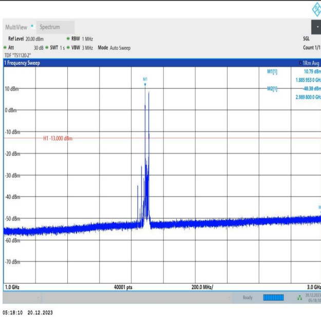
2-2-10MHz-15MHz-16QAM-16QAM-19005-19125-1RB#0-1RB #74-1000~3000MHz-PASS
