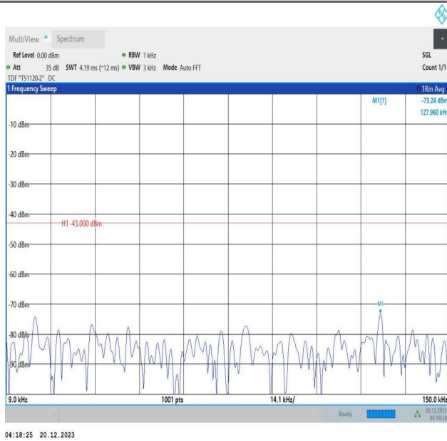
2-2-10MHz-15MHz-16QAM-16QAM-18829-18949-50RB#0-75 RB#0-0.009~0.15MHz-PASS
