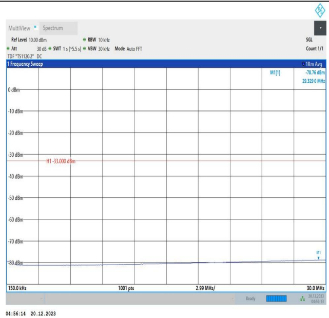
2-2-10MHz-15MHz-64QAM-64QAM-19005-19125-1RB#0-0RB #0-0.15~30MHz-PASS
