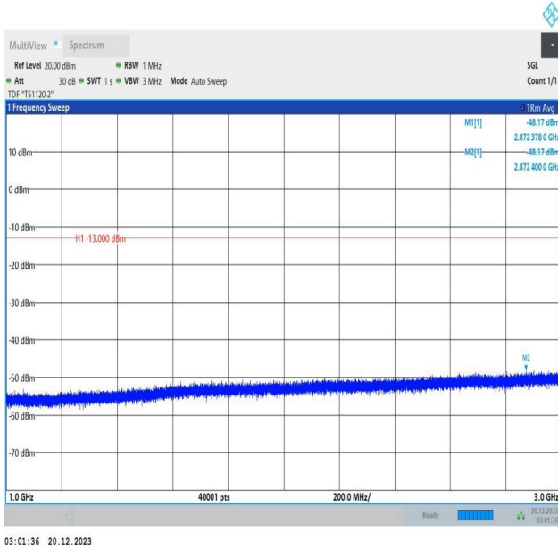
2-2-10MHz-15MHz-64QAM-64QAM-18653-18773-50RB#0-75 RB#0-1000~3000MHz-PASS
