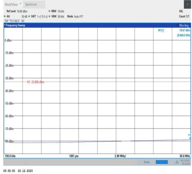
2-2-10MHz-15MHz-64QAM-64QAM-19005-19125-1RB#0-1RB #74-0.15~30MHz-PASS
