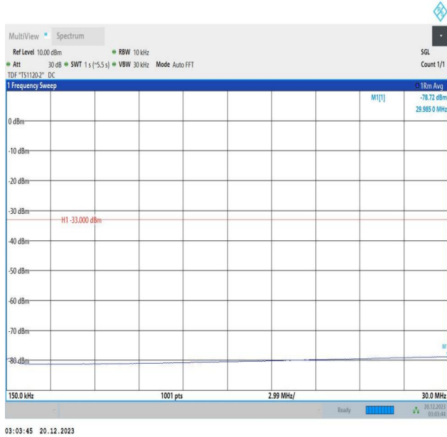
2-2-10MHz-15MHz-16QAM-16QAM-18829-18949-1RB#0-0RB #0-0.15~30MHz-PASS
