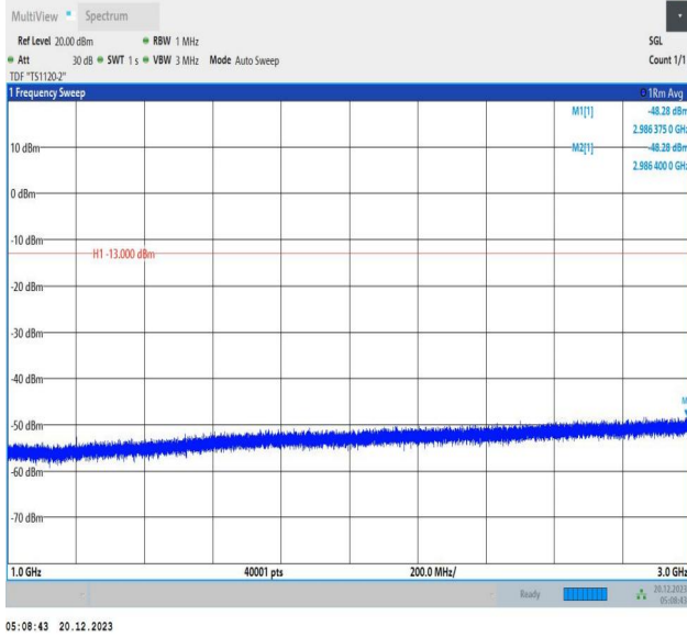
2-2-10MHz-15MHz-64QAM-64QAM-19005-19125-1RB#49-0R B#0-1000~3000MHz-PASS
