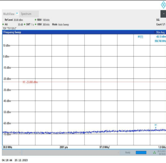
2-2-10MHz-15MHz-16QAM-16QAM-18829-18949-50RB#0-75 RB#0-30~1000MHz-PASS
