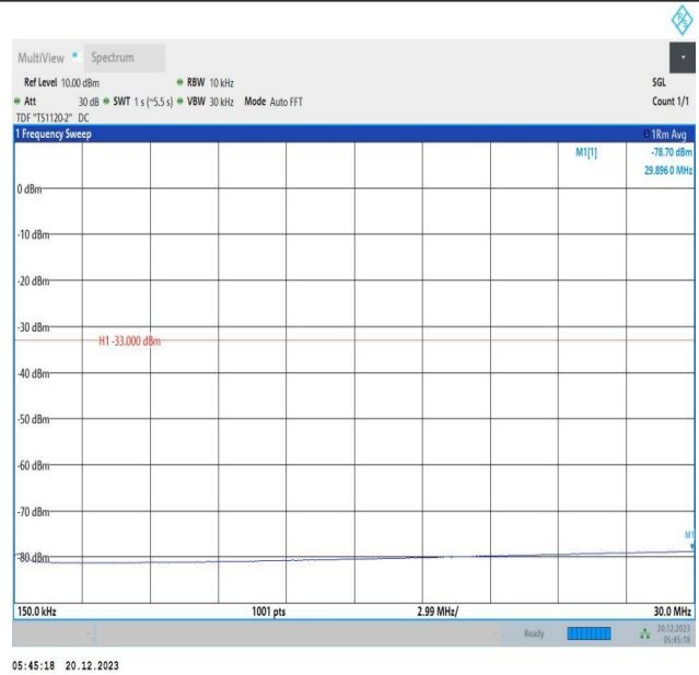
2-2-10MHz-15MHz-16QAM-16QAM-19005-19125-50RB#0-75 RB#0-0.15~30MHz-PASS
