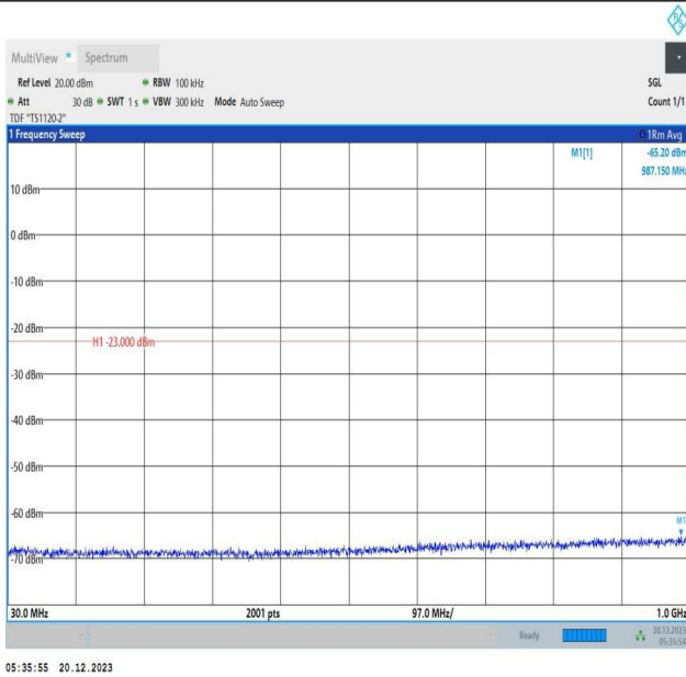
2-2-10MHz-15MHz-64QAM-64QAM-19005-19125-1RB#0-1RB #74-30~1000MHz-PASS
