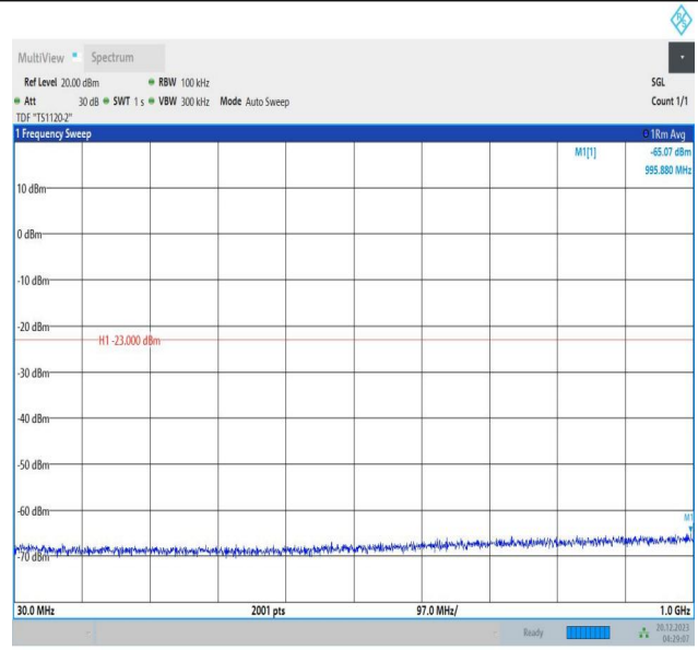
2-2-10MHz-15MHz-64QAM-64QAM-18829-18949-50RB#0-75 RB#0-30~1000MHz-PASS
