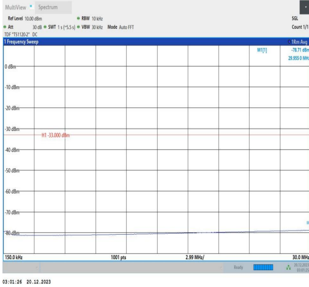
2-2-10MHz-15MHz-64QAM-64QAM-18653-18773-50RB#0-75 RB#0-0.15~30MHz-PASS
