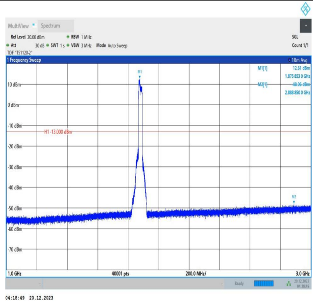
2-2-10MHz-15MHz-16QAM-16QAM-18829-18949-50RB#0-75 RB#0-1000~3000MHz-PASS
