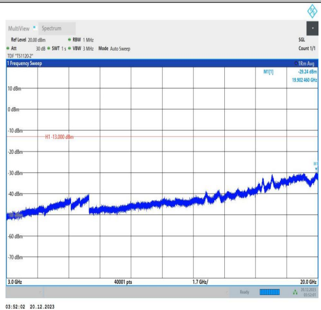
2-2-10MHz-15MHz-16QAM-16QAM-18829-18949-1RB#0-1RB #74-3000~20000MHz-PASS
