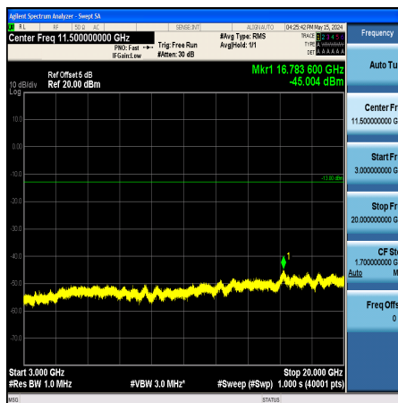
Band25_5MHz_16QAM_26665_1RB#0_3000~20000_3000~20000
