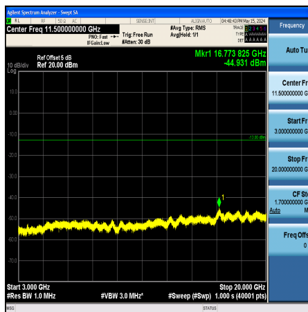
Band25_10MHz_QPSK_26090_1RB#0_3000~20000_3000~20000
