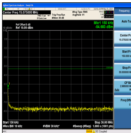
Band25_3MHz_QPSK_26365_1RB#0_0.15~30_0.15~30
