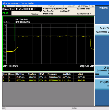
Band25_10MHz_QPSK_26090_50RB#0
