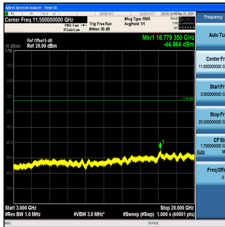
Band25_3MHz_16QAM_26055_1RB#0_3000~20000_3000~20000
