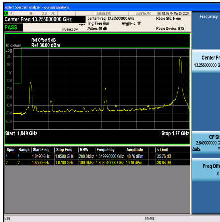
Band25_20MHz_QPSK_26140_1RB#99
