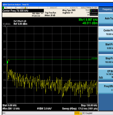
Band25_3MHz_QPSK_26365_1RB#0_0.009~0.15_0.009~0.15
