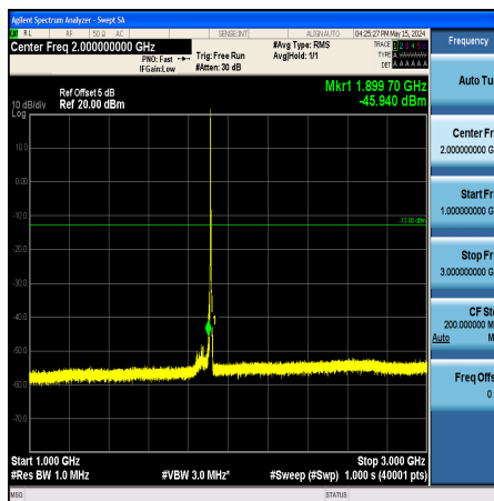
Band25_5MHz_16QAM_26665_1RB#0_1000~3000_1000~3000
