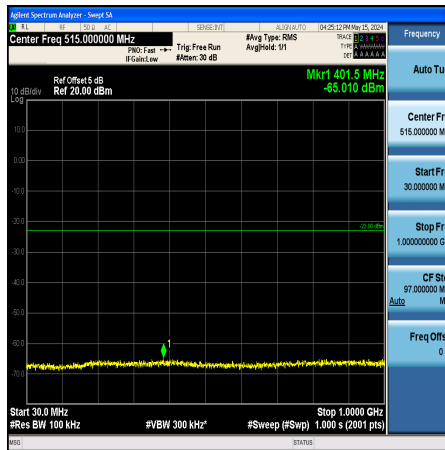
Band25_5MHz_16QAM_26665_1RB#0_30~1000_30~1000
