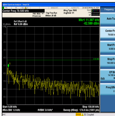
Band25_10MHz_16QAM_26090_1RB#0_0.009~0.15_0.009~0.15
