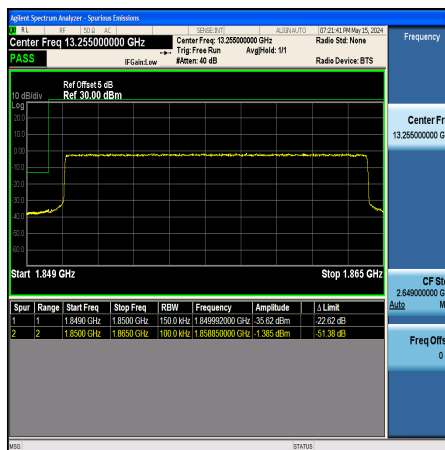
Band25_15MHz_QPSK_26115_75RB#0
