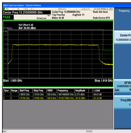
Band25_10MHz_QPSK_26640_50RB#0
