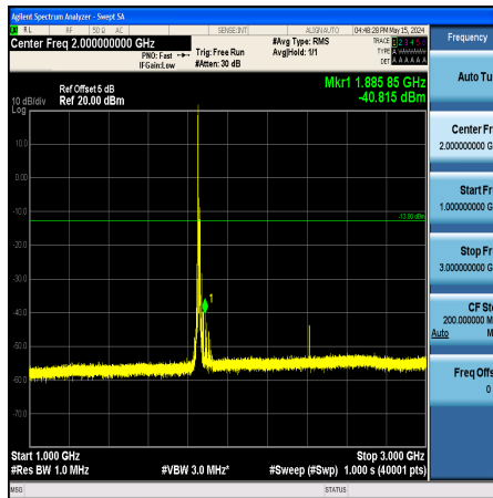
Band25_10MHz_QPSK_26090_1RB#0_1000~3000_1000~3000
