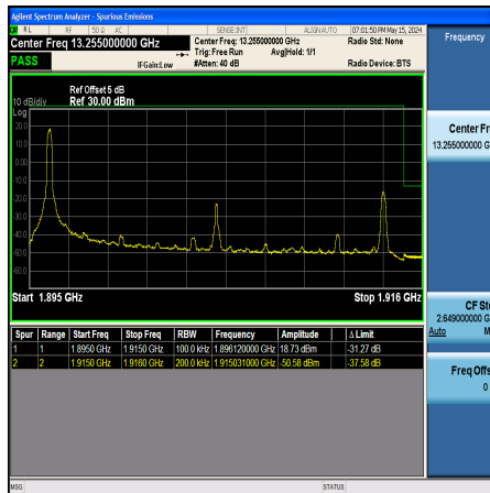
Band25_20MHz_16QAM_26590_1RB#0
