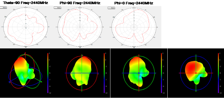
整机有源测试数据Active test data of the unit
