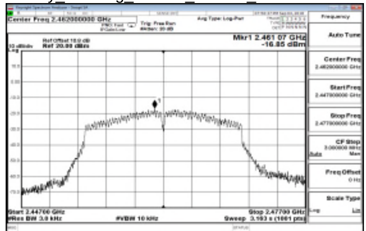
Power Density 802.11g 20MHz Chain0 2462MHz
