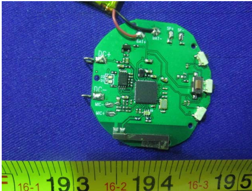
EUT –Headset Main Board Top View
