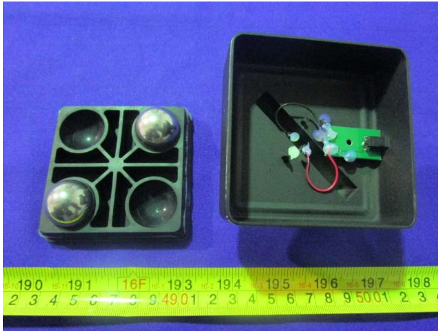
EUT –Charger Base Uncover View
