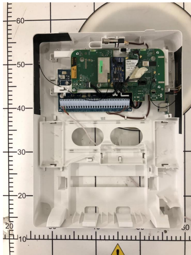
2. View of the DUT (Open)
