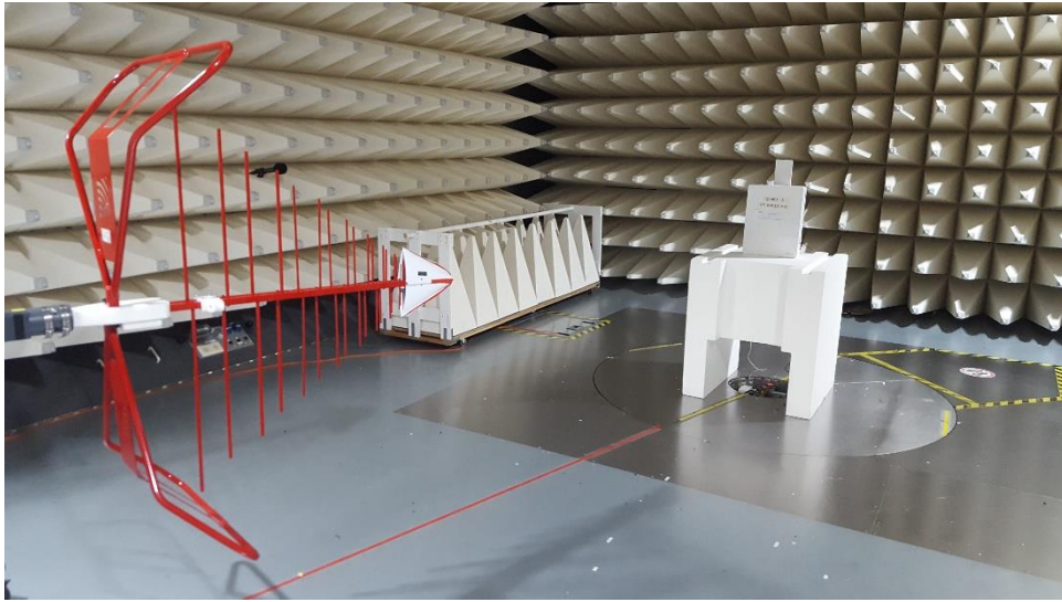
3. Radiated Emission test setup Low Range
