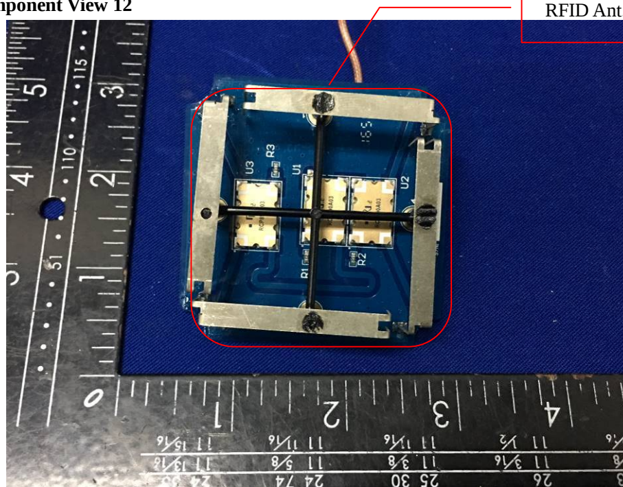
Solder Board-Component View 12
