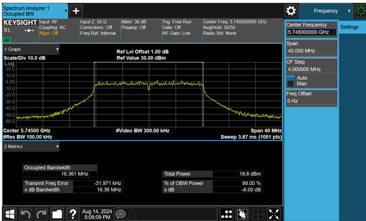
Figure 7: 802.11a, 5745MHz
