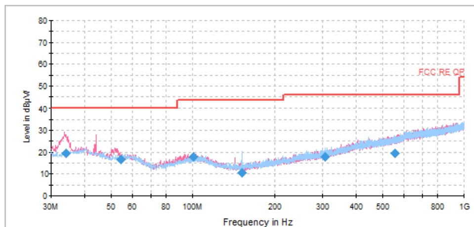
Radiated Emission from 30MHz to 1GHz
