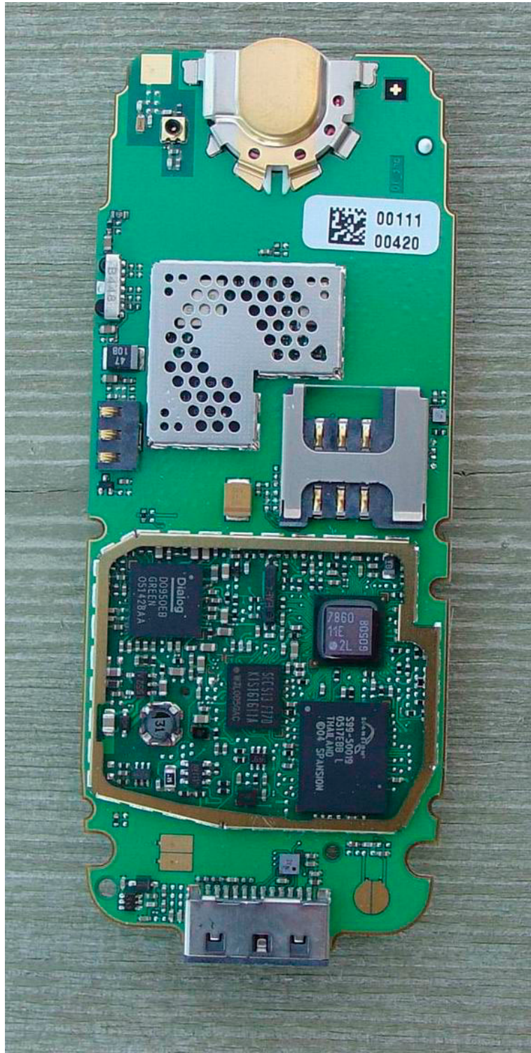
AX76 Back view repair lid installed
