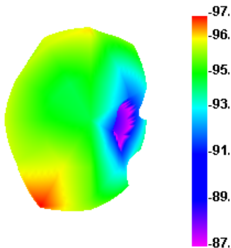
Bluetooth 39 TIS
