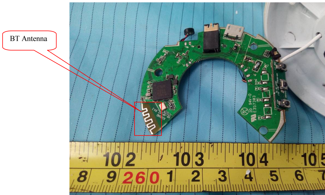
EUT – Mainboard 1 Top View
