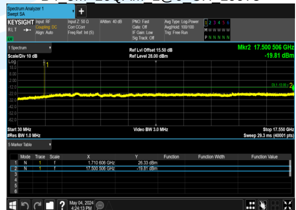
B4_5M_16QAM_1@0_CH_19975
