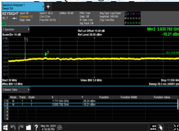
B4_15M_QPSK_1@0_CH_20175
