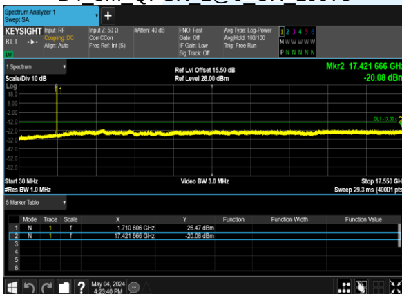
B4_5M_QPSK_1@0_CH_19975
