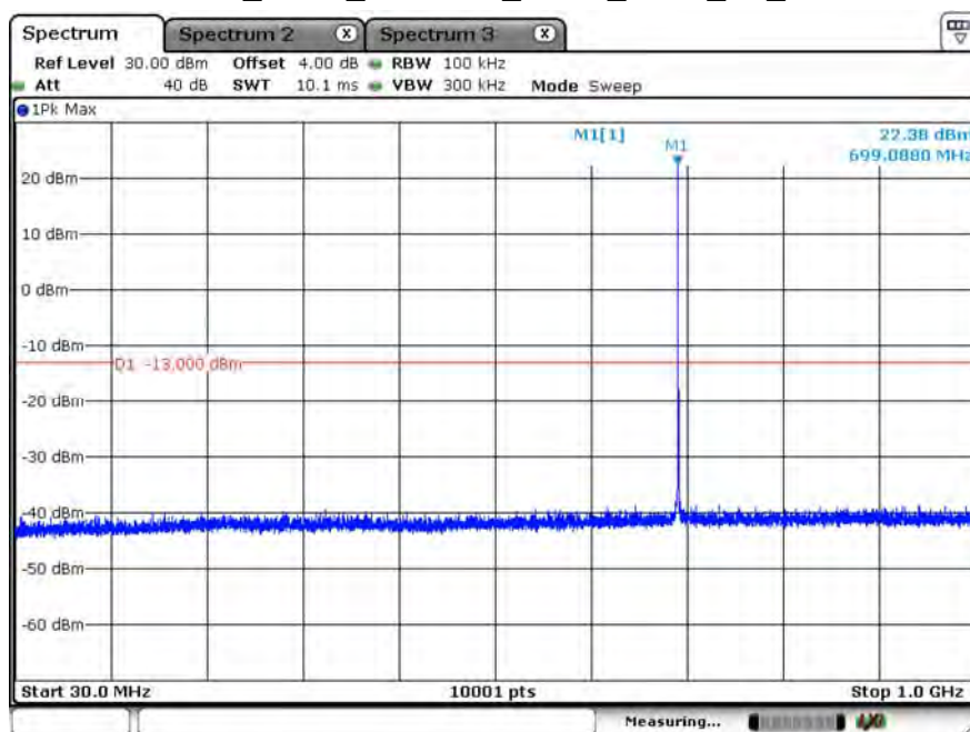
B12_3.75K_CH23012_BPSK_1RB0_TX_1
