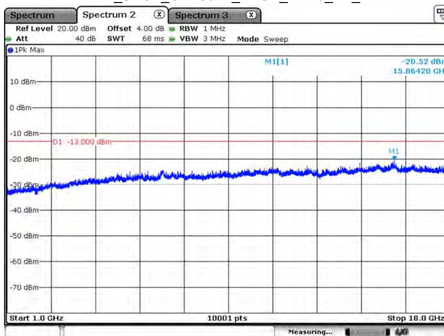
B12_3.75K_CH23012_BPSK_1RB0_TX_2
