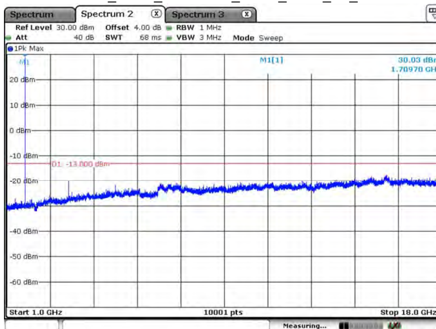
B66_3.75K_CH131974_BPSK_1RB0_TX_2
