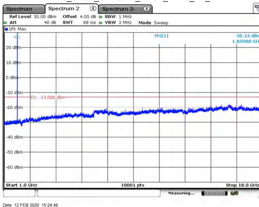
B25_3.75K_CH26042_BPSK_1RB0_TX_2
