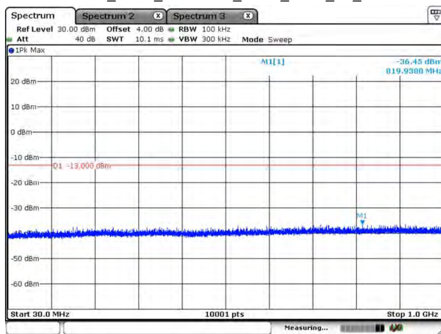
B66_3.75K_CH131974_BPSK_1RB0_TX_1
