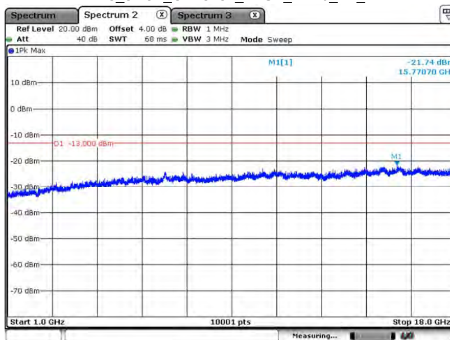
B13_3.75K_CH23182_BPSK_1RB0_TX_2
