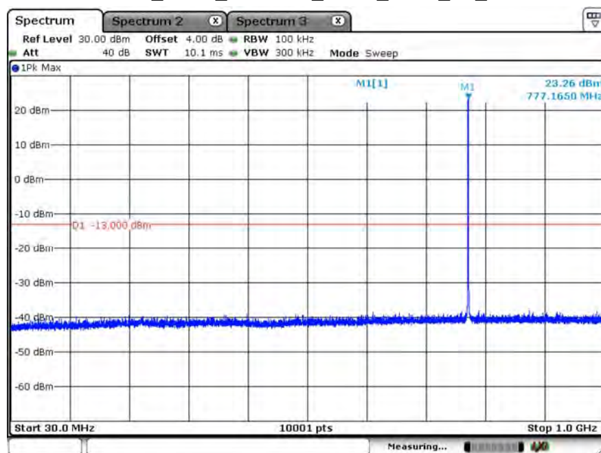
B13_3.75K_CH23182_BPSK_1RB0_TX_1
