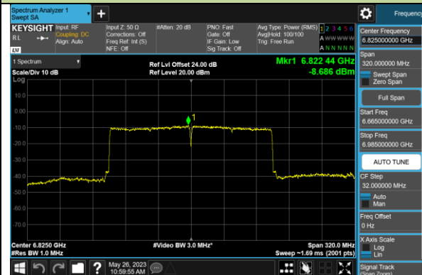
Channel 175 (6825MHz)
