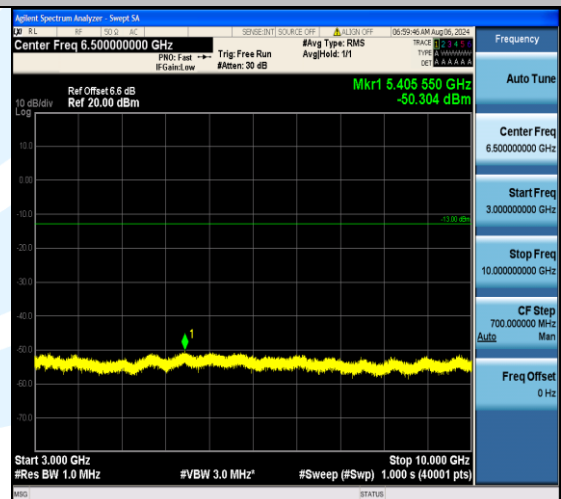
Band5_10MHz_QPSK_20525_50RB#0_3000~10000_3000~10000
