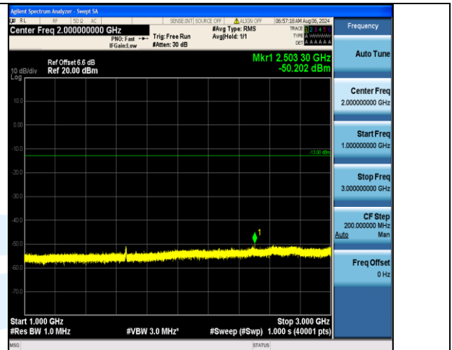
Band5_10MHz_QPSK_20450_50RB#0_1000~3000_1000~3000
