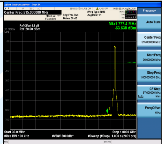
Band5_10MHz_QPSK_20525_50RB#0_30~1000_30~1000
