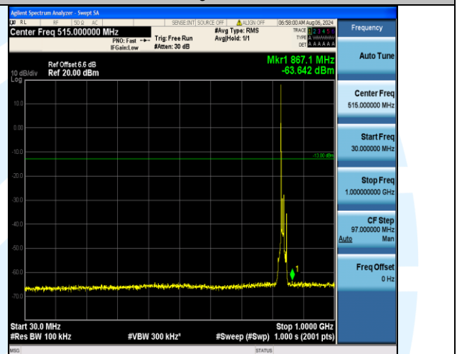
Band5_10MHz_QPSK_20525_1RB#0_30~1000_30~1000
