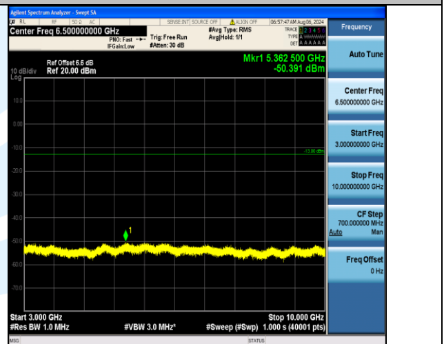
Band5_10MHz_16QAM_20450_50RB#0_3000~10000_3000~10000
