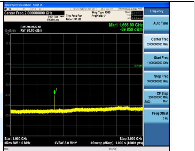
Band5_10MHz_16QAM_20450_1RB#49_1000~3000_1000~3000
