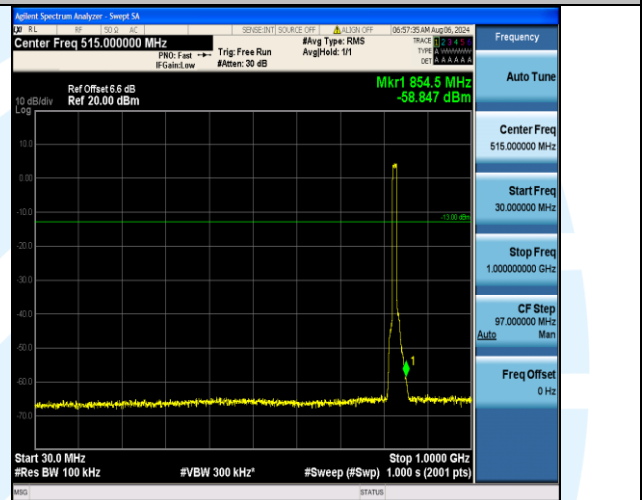
Band5_10MHz_16QAM_20450_50RB#0_30~1000_30~1000
