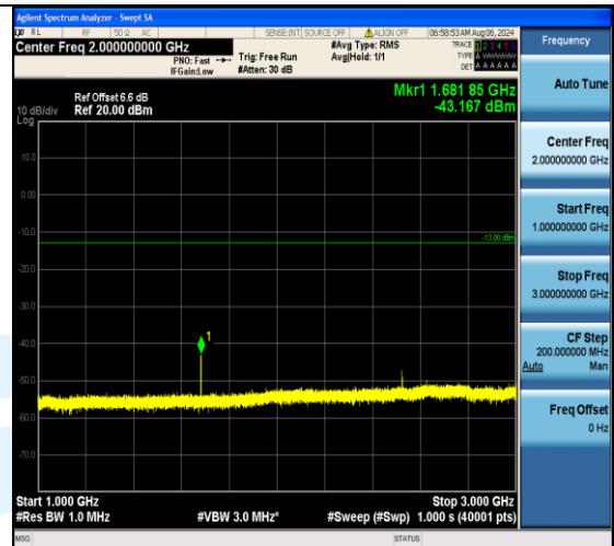
Band5_10MHz_QPSK_20525_1RB#49_1000~3000_1000~3000
