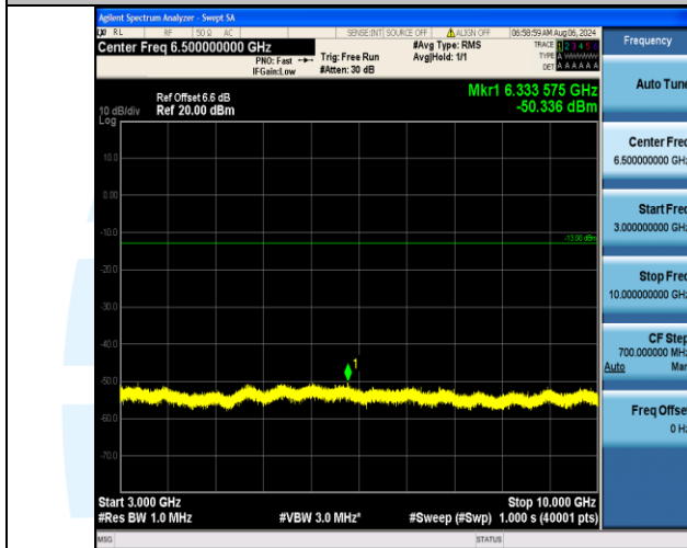
Band5_10MHz_QPSK_20525_1RB#49_3000~10000_3000~10000
