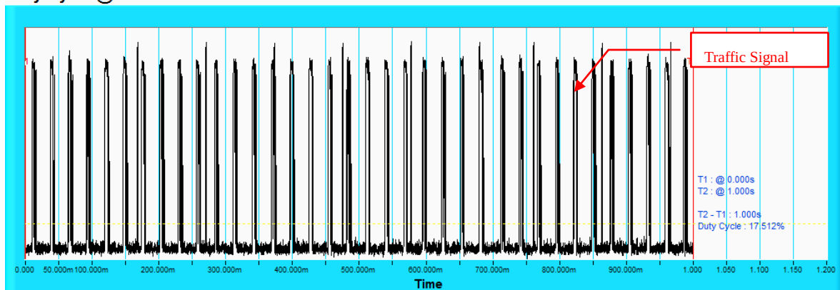
Duty Cycle @ CH102
