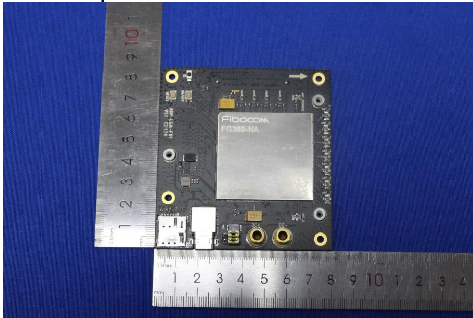
Test PCB board photo FG360-NA
