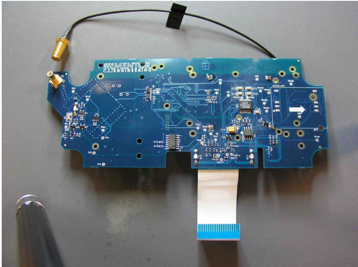
RFM Assembly Bottom
