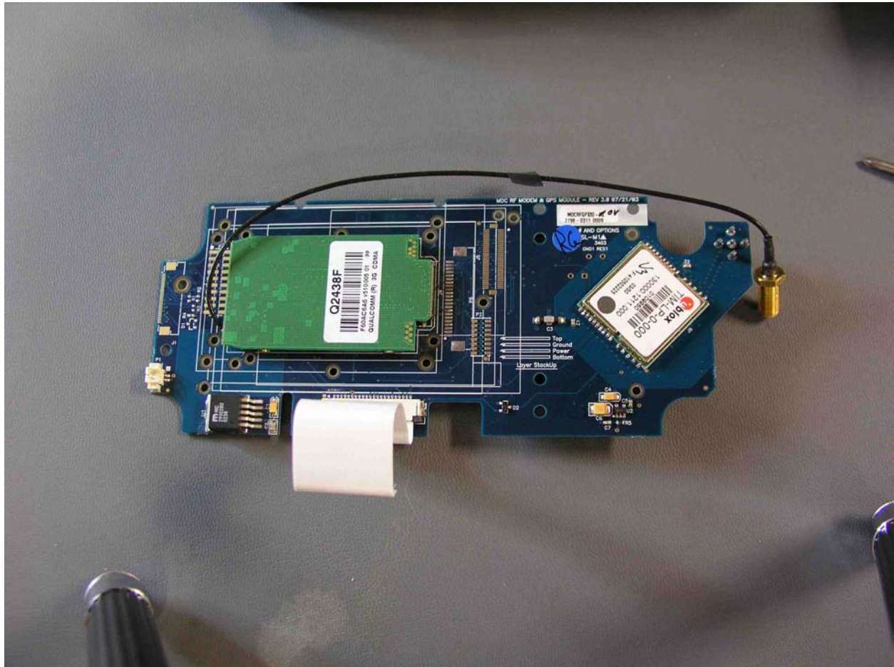
RFM Assembly Top
