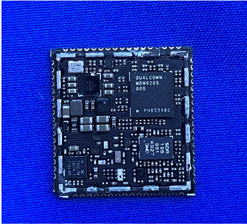
(1) EUT Photo
