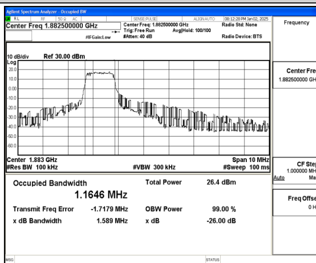
Band25-5MHz-16QAM-26365-6-0-Low-1.1646-1.589-PASS
