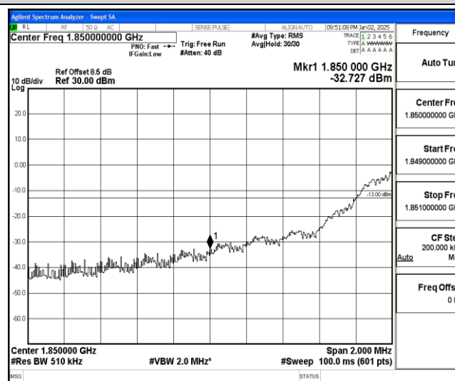
Band25-20MHz-16QAM-26140-6-0-Low--32.73-PASS
