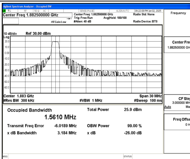
Band25-15MHz-QPSK-26365-6-0-Low-1.5610-3.184-PASS
