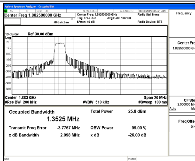
Band25-10MHz-16QAM-26365-6-0-Low-1.3525-2.098-PASS
