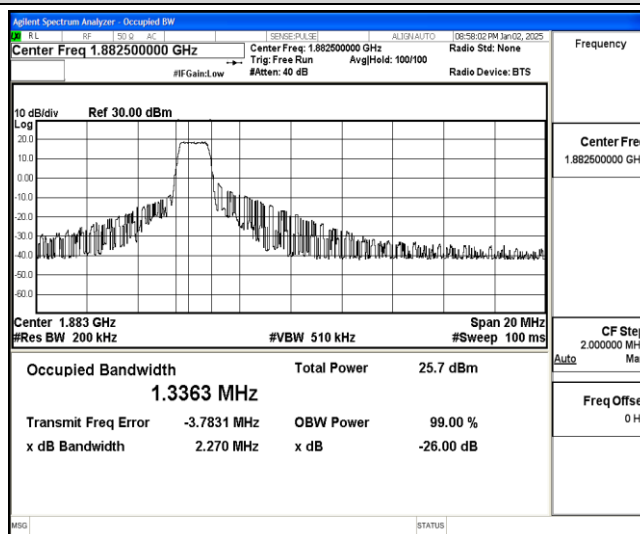
Band25-10MHz-QPSK-26365-6-0-Low-1.3363-2.270-PASS
