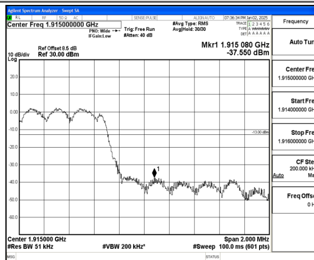
Band25-3MHz-16QAM-26675-6-0-High--37.55-PASS
