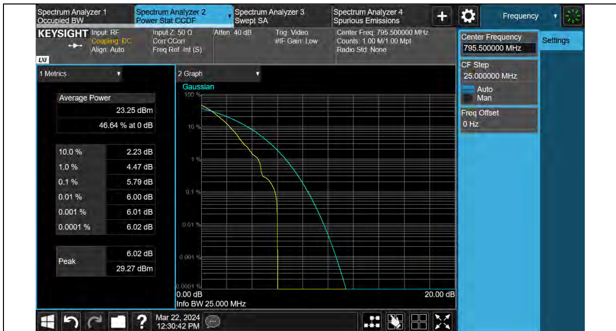
Band14-5MHz-16QAM-23305
