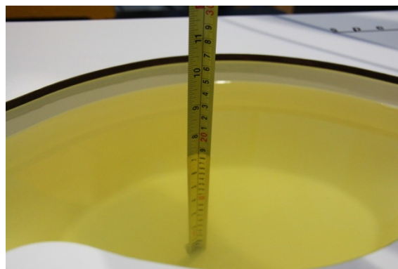
Liquid depth in the body phantom (1750MHz)
